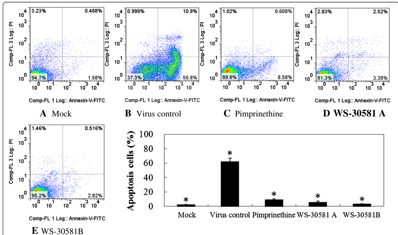
Figure 6 The inhibitory effects of pimprinethine, WS-30581 A and WS-30581 B on EV71-induced apoptosis. RD cells were left untreated (A) or were infected with 100 TCID 50 of EV71, after viral adsorption, RD cells were incubated in the absence (B) or presence of 80 μM pimprinethine (C) , 40 μM WS-30581 A (D) and 40 μM WS-30581 B (E) for 36–48 h, the cells were stained with Annexin-V- fluorescein and propidium iodide and measured using flow cytometry. Values are represented as means ± SDs. *P < 0.05, compared with virus control group.
