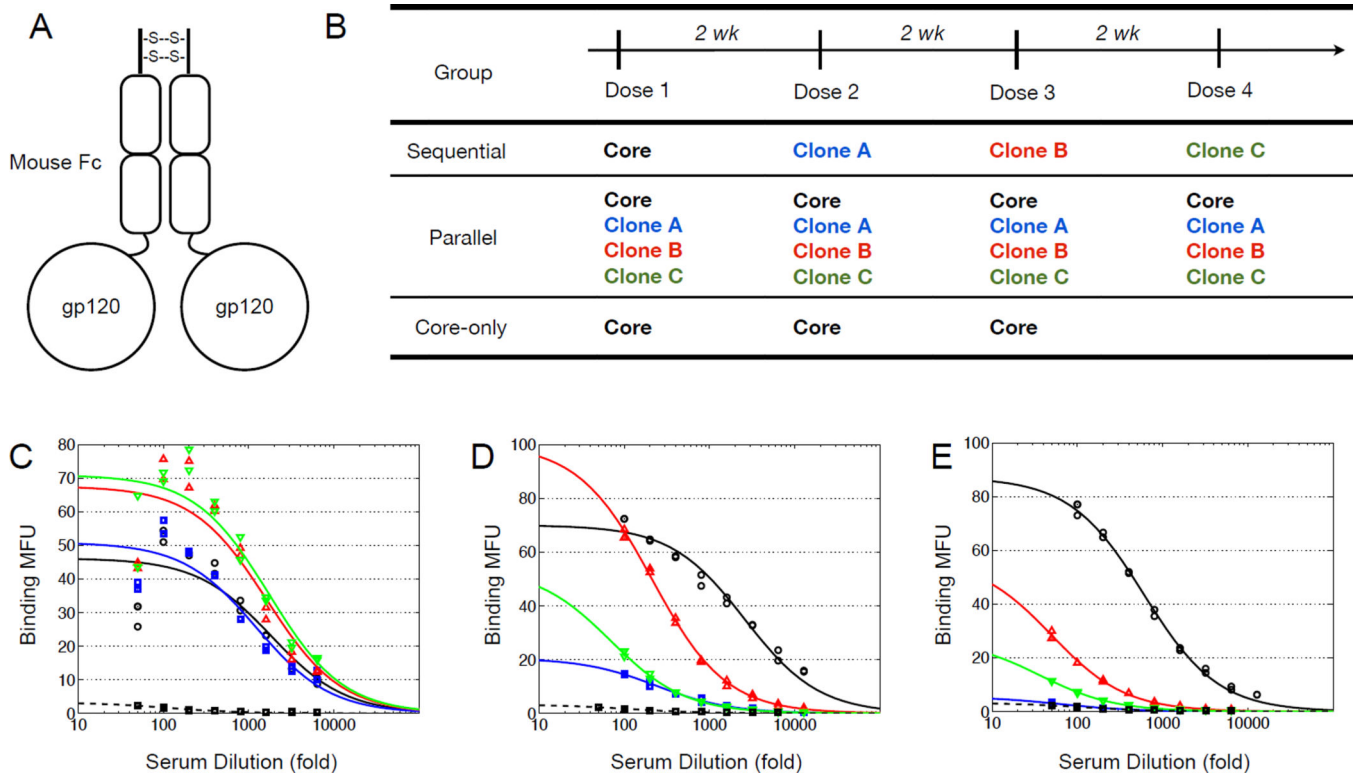
Figure 5. Immunization of mice with variant immunogens
