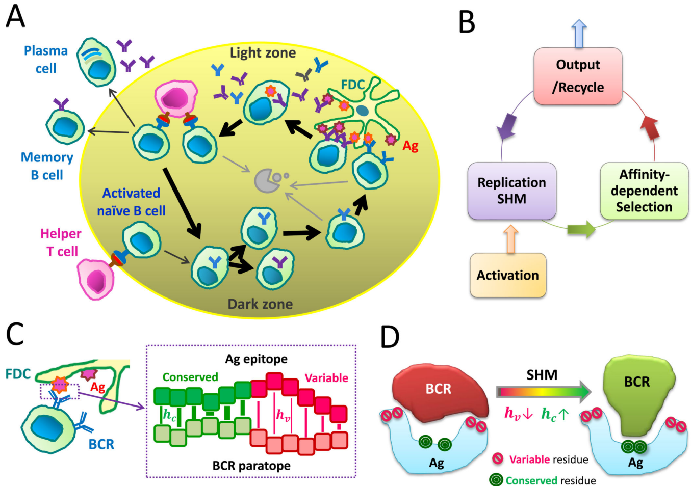
Figure 1. Schematic depiction of in silico model
