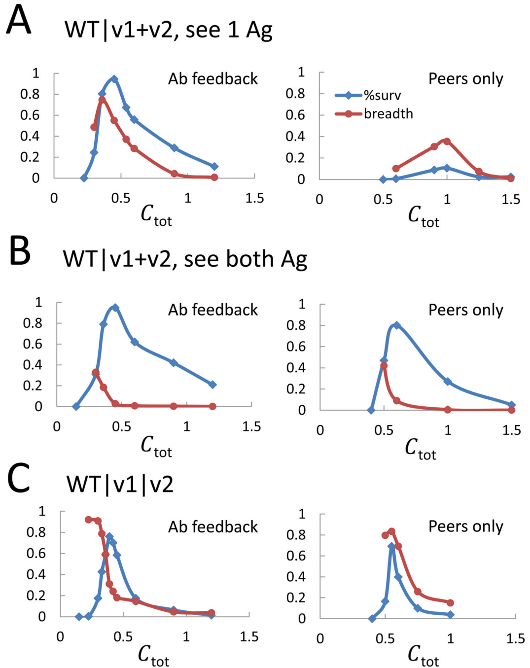
Figure 2. Concentration dependence of GC survival and antibody breadth in “WT first” schemes
