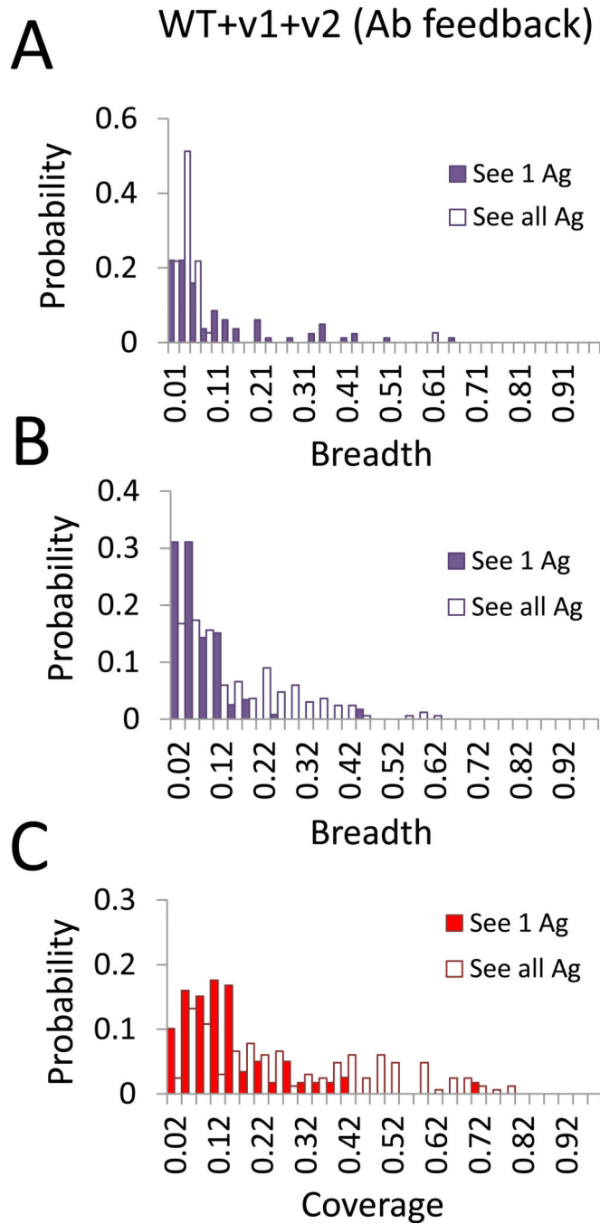
Figure 3. Distribution of breadth of individual antibodies and their total coverage for surviving GCs in scheme I—WT+v1+v2
