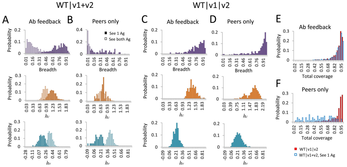
Figure 4. Comparison of statistics for surviving GCs in Scheme II—WT|v1+v2 and Scheme III—WT|v1|v2
