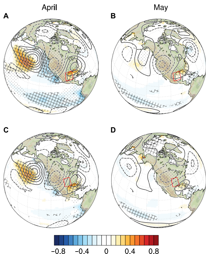
Fig. 3. Large-scale patterns controlling the low-level jet from the Gulf of Mexico and moisture over the SGP. Linear regression patterns of Z_{500} ' (contour) and SSTAs (shaded areas) onto (A and B) V925_S and (C and D) MFC925 for April (left) and May (right). The contour intervals are 0.08 K for SSTa and 8 m for Z_{500} '. The stippled (cross-hatched) area indicates values for which the local null hypothesis of zero regression can be rejected at the 95% level for Z_{500} ' (SSTA), based on a Student's t test with 61 degrees of freedom. Long-term linear trends were removed before any statistical analysis.
