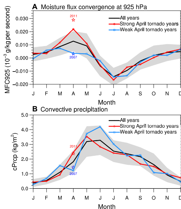
Fig. 4. Thermodynamic variables during strong and weak April tornado years. Monthly climatologies of the (A) MFC925 and (B) cPrpc over the SGP from all years (black line), strong April tornado years (red line), and weak April tornado years (blue line). The strong (weak) April tornado years are selected on the basis of 1.5 (–1.1) SDs. The selected strong years are 1957, 1964, 1979, 1982, 1991, and 2011, and the weak years are 1959, 1987, 1992, 1997, and 2007. MFC925 is obtained from NCEP1 for 1954–2016, and cPrpc is obtained from the NARR dataset for 1979–2016. Gray-shaded area encompasses 1 SD of all years. Because of the different time frames that each dataset covers, missing years are omitted from the composite mean calculation. Two representative strong and weak tornado years are indicated by the red and blue stars, respectively.
