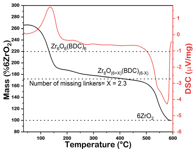
Fig. 3 Calculation of the number of missing BDC linkers per hexa-zirconium node. The final mass of 6ZrO_2 is taken as 100 and that of the dehydroxylated perfect MOF before thermal decomposition is taken as 220.
