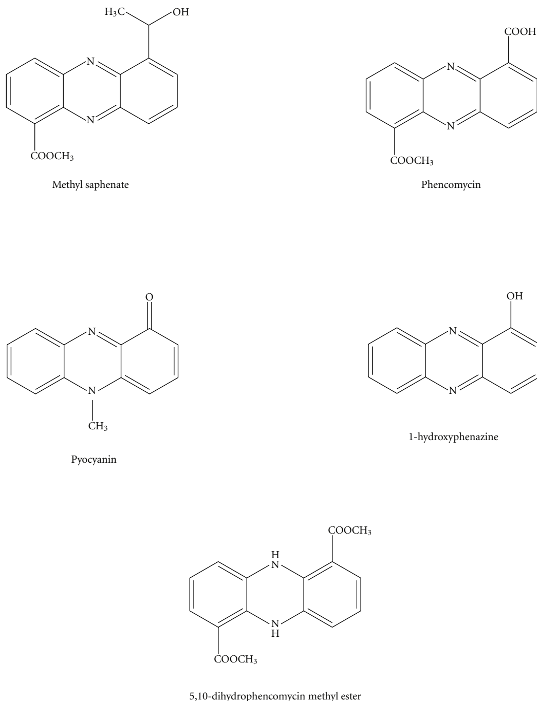
FIGURE 4: Phenazine derivatives.
