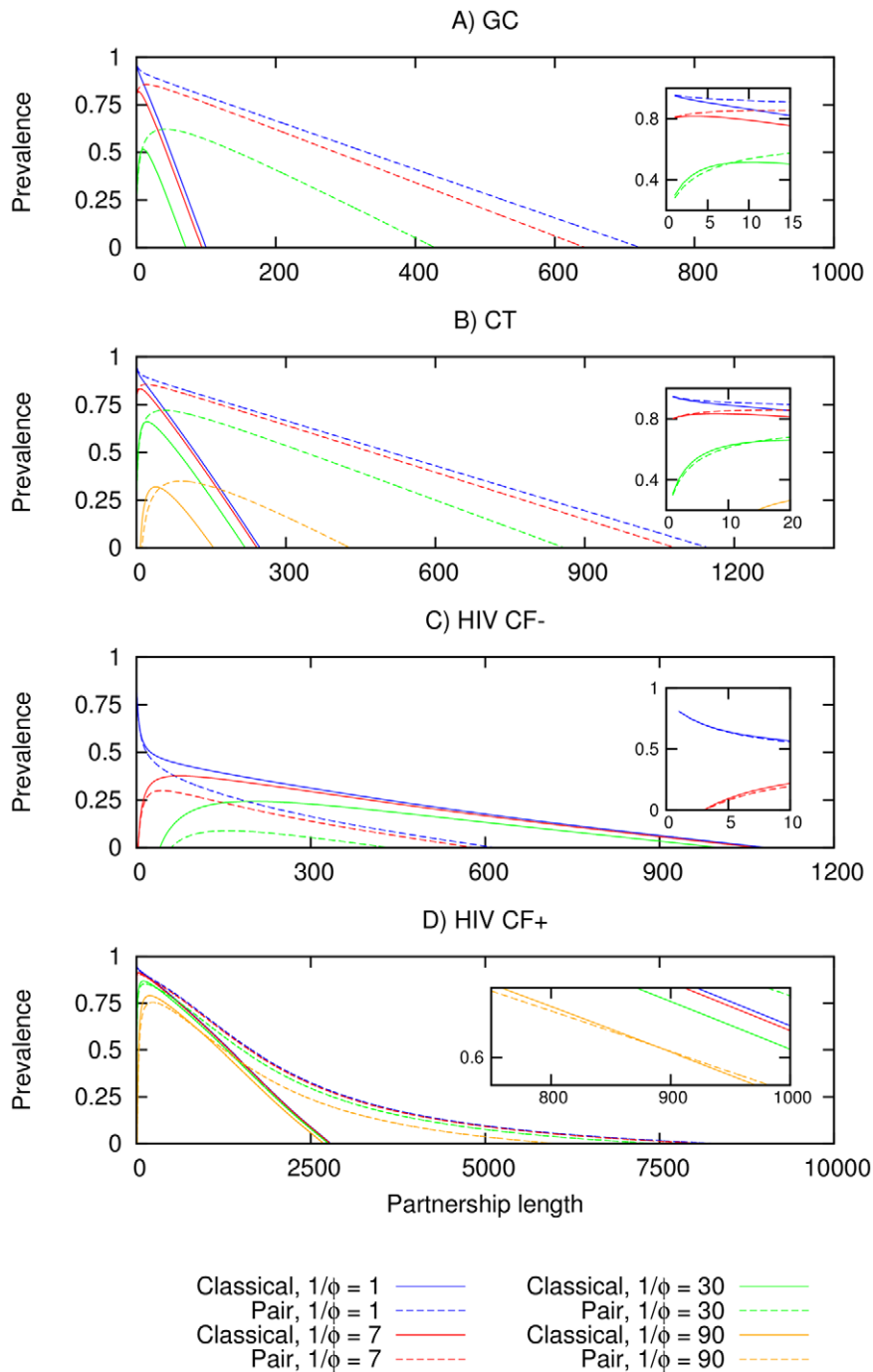
Figure 1. Predictions from the classical and pair model formulations for the steady-state \pi^s of GC/CT (A and B), and the peak \pi^p of HIV with and without cofactor enhancement (C and D). The horizontal axes give partnership length in days while the vertical axes give \pi . The different lines denote predictions from using gap lengths ( 1/\beta ) of 1 day, 7 days, 30 days and 90 days. The inset in each figure magnifies crossover point, if any, in the region where the classical and pair models diverge in \pi predictions. Models in (A) and (C) are unable to provide predictions at a gap length of 90 days. doi:10.1371/journal.pone.0039575.g001
