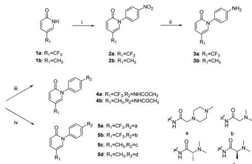
Scheme 1 Synthetic route to compounds 4a–4b and 5a–5d . Reagents and conditions: (i) MeCN, K_2CO_3 , 85 °C. (ii) SnCl_2 \cdot 2H_2O , conc. HCl, 40 °C. (iii) Ac_2O , 125 °C. (iv) Acid derivative, HATU, DIPEA, 0–25 °C.
