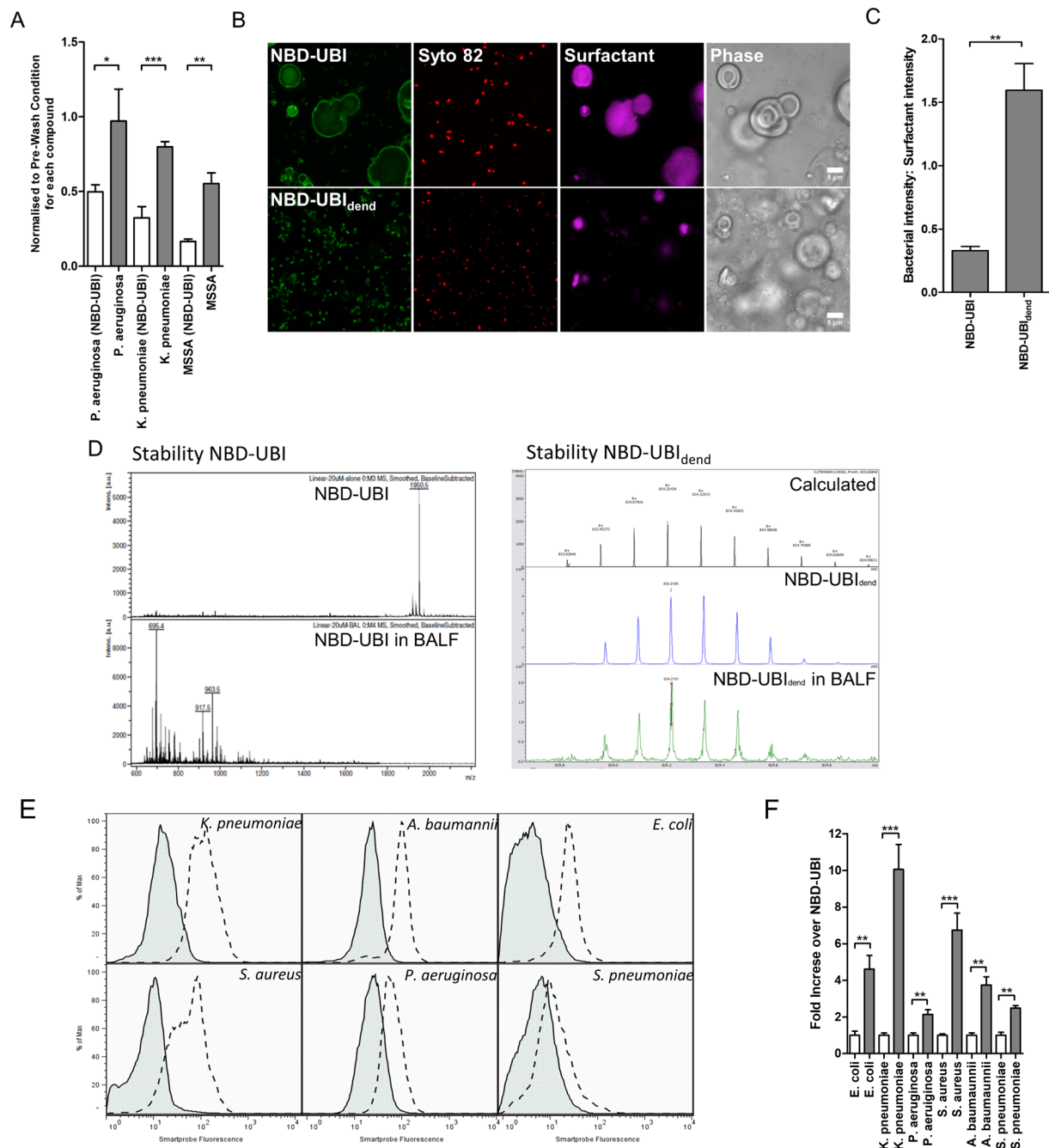
Figure 3. NBD-UBI dend has greater affinity and demonstrates improved signal-to-noise when labelling bacteria in pulmonary surfactant than the linear NBD-UBI and shows stability in ARDS BALF. (A) Quantification of retained fluorescence following a wash and re-imaging on a benchtop confocal microscope. Each bacterial strain and compound were normalised to their pre-wash fluorescence intensities (bacteria were incubated with NBD-UBI at 15 \mu M or equimolar concentration of NBD-UBI dend at 5 \mu M). Bars represent means ( \pm SEM) of independent experiments where at least three fields of view were assessed, and analysed by a Student's t-test, * p < 0.05 , ** p < 0.01 , *** p < 0.001 . (B) Representative images of P. aeruginosa imaged in the presence of synthetic pulmonary surfactant. Green panels show either NBD-UBI 10 \mu M or NBD-UBI dend 3.3 \mu M with red panels showing Syto82 counterstaining, purple panels showing synthetic surfactant and phase contrast images demonstrating surfactant vesicles. (C) Fluorescence quantification of P. aeruginosa imaged with NBD-UBI at 10 \mu M or NBD-UBI dend at 3.3 \mu M in the presence of fluorescently labelled high-density surfactant vesicles. Data represents the mean fluorescence of the NBD channel on bacteria compared to surfactant and show a significantly higher bacteria:surfactant fluorescence intensity for NBD-UBI dend than NBD-UBI. Bars represent means ( \pm SEM) of three independent experiments where at least three fields of view were assessed, analyses by Student's t-test, ** p < 0.01 . (D) Stability of compounds in saline and ARDS BALF demonstrating breakdown of NBD-UBI in ARDS BALF when analysed by MALDI-TOF MS (left panel) the presence of NBD-UBI dend in ARDS BALF when assessed by FTMS (right panel). (E) Representative flow histograms for bacteria when incubated with NBD-UBI (grey histograms) at 15 \mu M or NBD-UBI dend 5 \mu M (dotted line) demonstrating a
