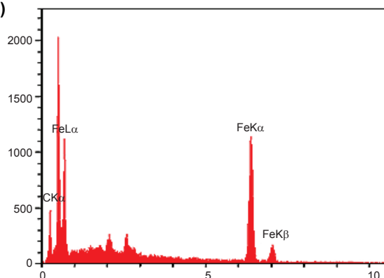
Figure 1. Characterization of \text{Fe}_3\text{O}_4 @ \beta -CD nanoparticles. A) The SEM image and the size distribution histogram B) EDS analysis.
