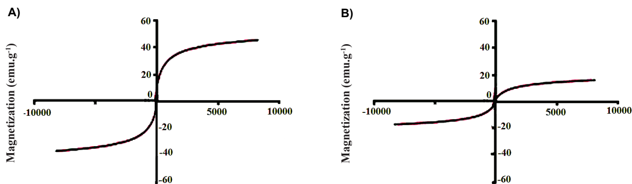
Figure 3. The magnetic hysteresis loop curves .A) \text{Fe}_3\text{O}_4@β\text{-CD} nanoparticles and B) PLA/ \text{Fe}_3\text{O}_4@β\text{-CD} / F. angulata .extract nanofibrous nanocomposite.
