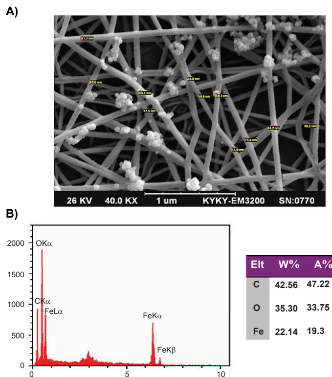
Figure 2. Characterization of PLA/ \text{Fe}_3\text{O}_4 @ \beta -CD/ F. angulate .extract nanofibrous nanocomposite. A) SEM images, B) EDS analysis.
