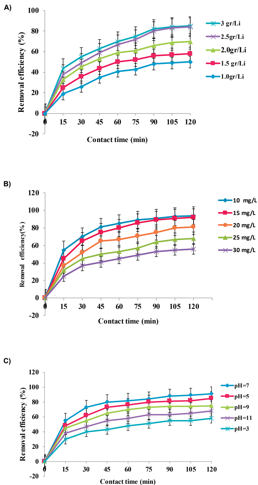
Figure 4. Impact of parameters on adsorption of diazinon onto PLA/Fe 3 O 4 @β-CD nanofibrous nanocomposite . A) Effect of adsorbent dosage and B) Effect of initial concentration of diazinon. C) Effect of initial pH on the adsorption of diazinon onto PLA/Fe 3 O 4 @β-CD nanofibrous nanocomposite .xlsx
