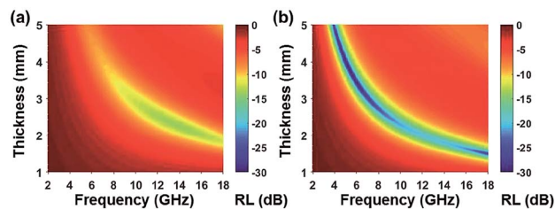
Fig. 11 (a) Reflection loss mapping of FCI and (b) RGO-coated FCI with absorbers thickness from 1 mm to 5 mm in the frequency range of 2.0 – 18.0 GHz 66 – reproduced by permission of The Royal Society of Chemistry.
