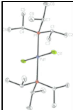
Fig. 1. A view of the title molecule, showing the atom-labelling scheme. Displacement ellipsoids are drawn at the 50% probability level and H atoms have been omitted for clarity. Unlabelled atoms are related to labelled atoms by the symmetry operation (1-x, 1-y, -z).
