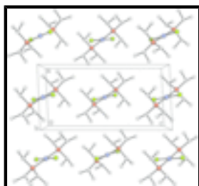
Fig. 2. Crystal packing of the title compound, viewed approximately along the b axis.
