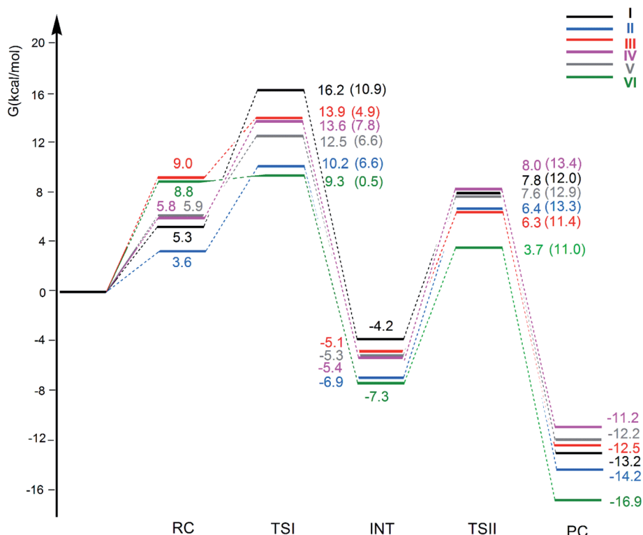
Fig. 4 Free energy reaction profile for the CO 2 insertion into the Au–Al bond in the [ t Bu 3 PAuAl(NON')] (I, black lines), [ t Bu 3 PAuAl(SiNON')] (II, blue lines), [ t Bu 3 PAuAl(NCCN')] (III, red lines), [ t Bu 3 PAuAl(D ip PBDI-H')] (IV, violet lines), [ t Bu 3 PAuAl(CAA')] (V, grey lines) and [ t Bu 3 PAuAl(C(CSiH 3 ) 2 CH 2 ) 2 ] (VI, green lines) complexes. ΔG values refer to the energy of the separated reactants taken as zero. Activation free energy barriers are reported in parentheses. The results for [ t Bu 3 PAu] and [ t Bu 3 PAuII] have been taken and adapted from ref. 33 and 45.
