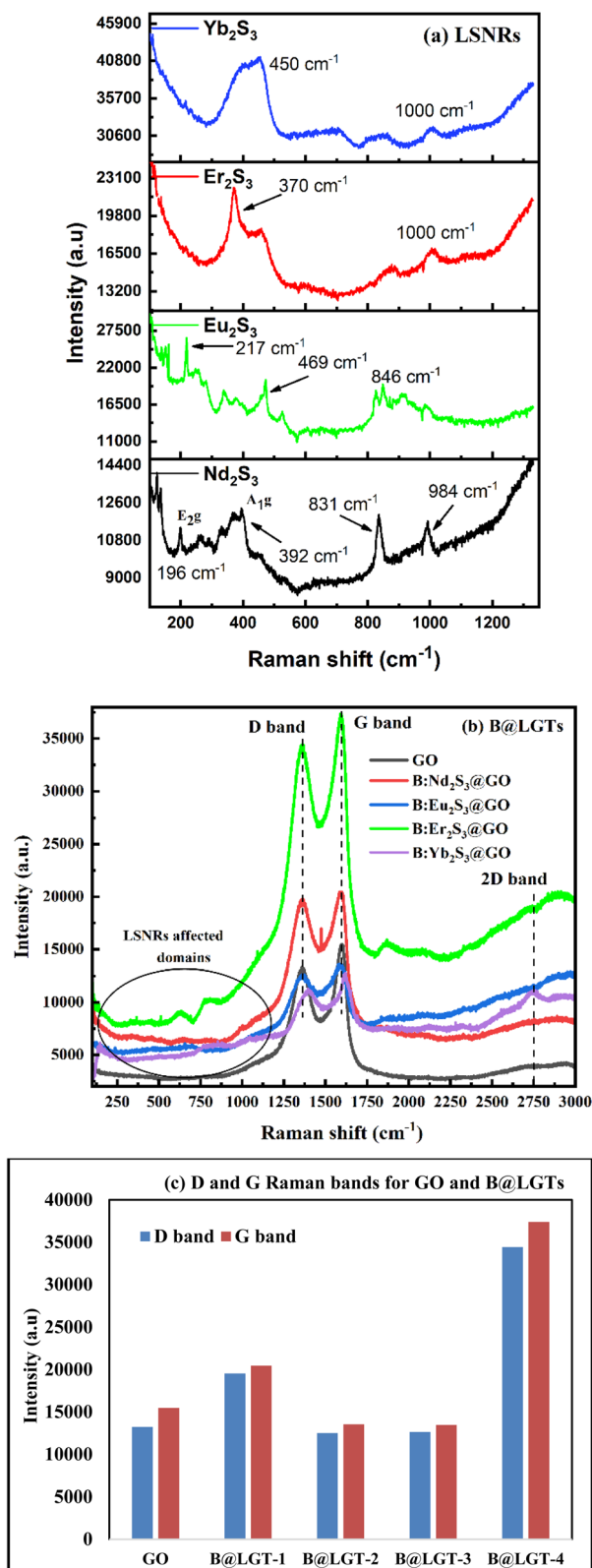
Fig. 11 Raman spectra for (a) LSNRs and (b) GO and B@LGTs elucidated the (c) D and G band intensities with I_D/I_G < 1 .
