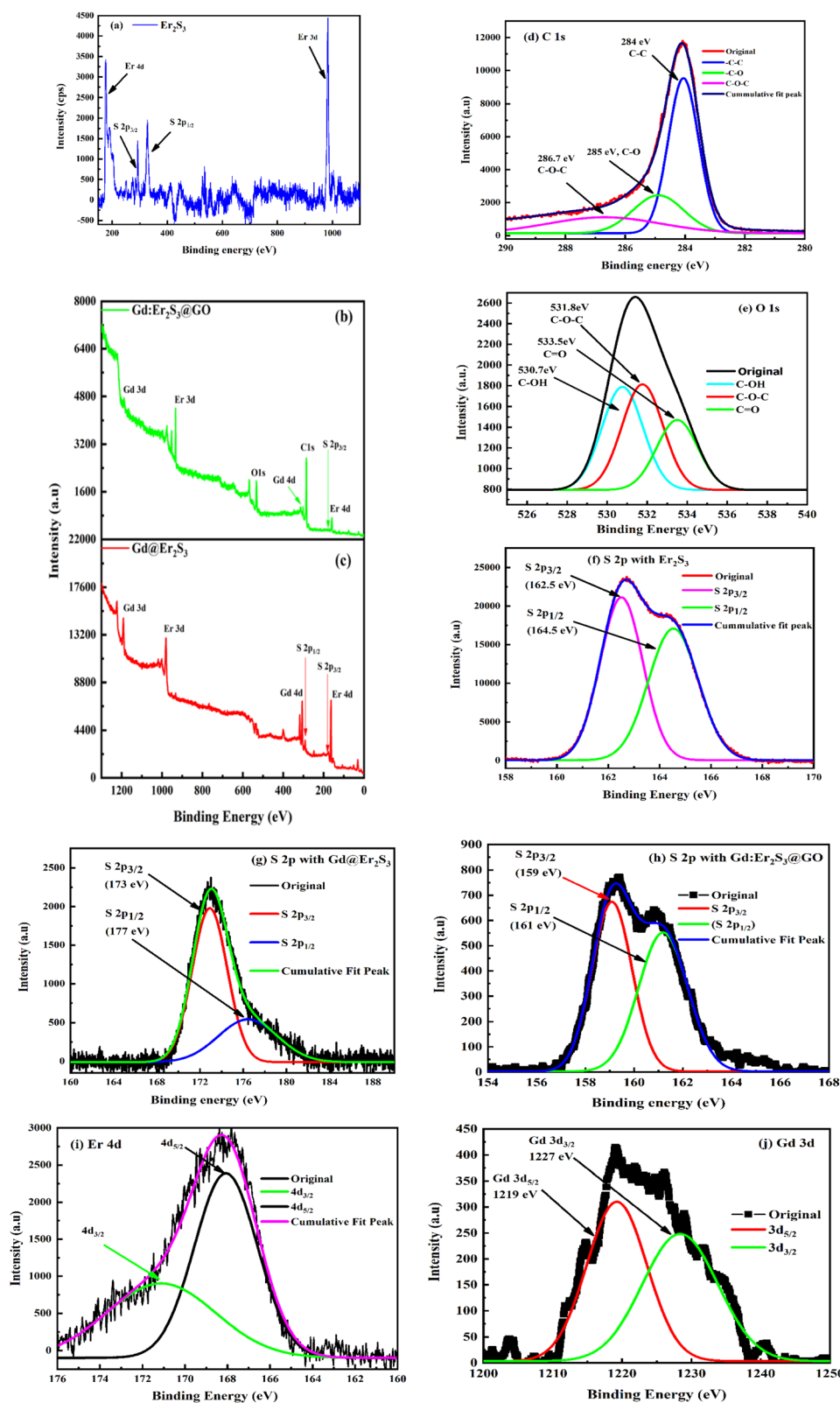
Fig. 13 XPS spectra: (a–c) survey scan for \text{B}@\text{Er}_2\text{S}_3 and \text{B}@\text{Er}_2\text{S}_3@\text{GO} ; (d) C 1s and (e) O 1s of \text{B}@\text{Er}_2\text{S}_3@\text{GO} ; (f–h) S 2p states; (i) Er 4d 3/2 and 4d 5/2 and (j) Gd 3d 3/2 and Gd 3d 5/2 .
