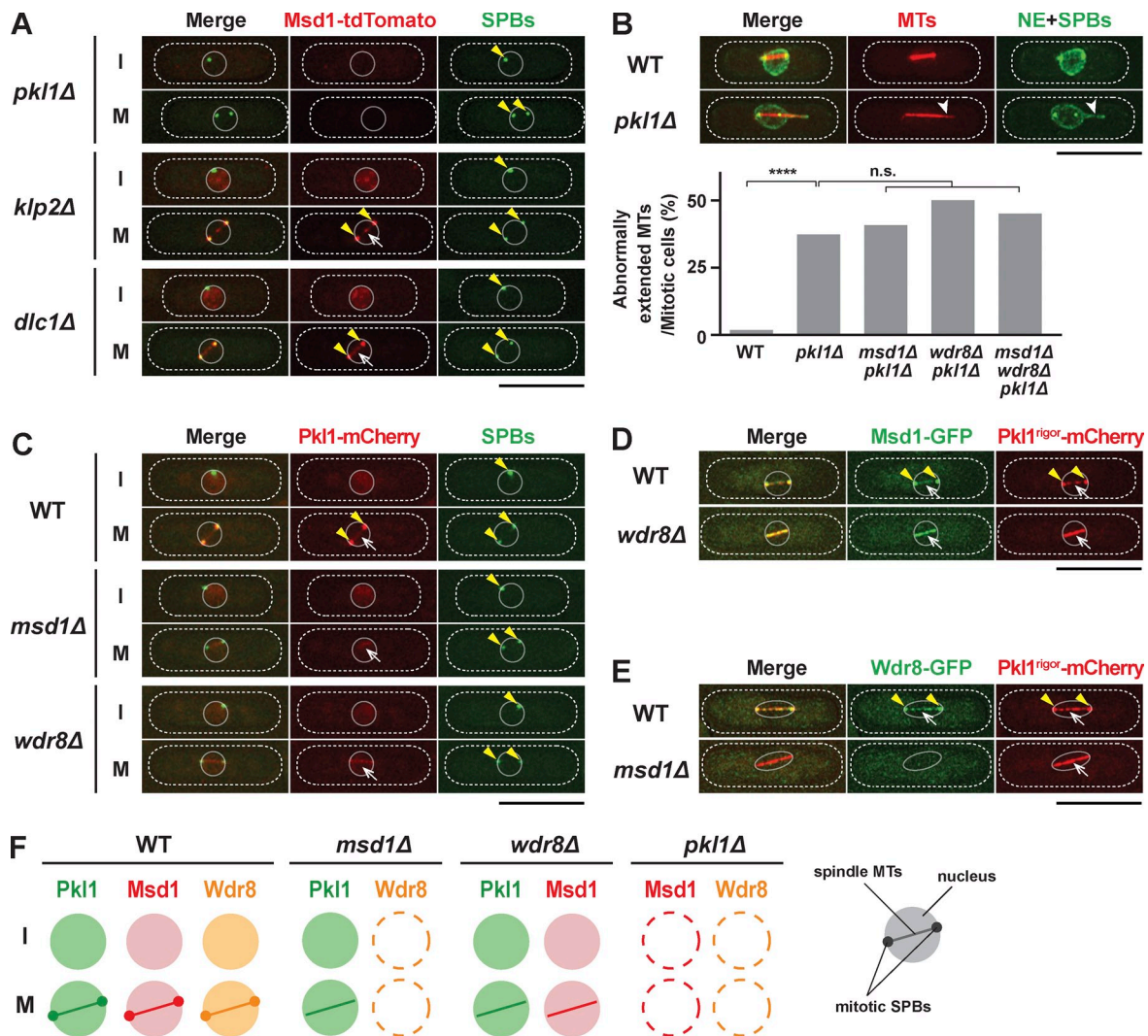
Figure 2. Msd1 and Wdr8 act together with Pk1/kinesin-14 for the anchorage of spindle microtubules to the SPB. (A) SPB localization of Msd1 requires Pk1/kinesin-14. Localization of Msd1-tdTomato and GFP-Alp4 (SPBs) in pk11Δ , klp2Δ , or dlc1Δ mutant cells during interphase (I) or mitosis (M) is shown. Cells were grown in rich media at 27°C. Note that Msd1 not only is localized to the mitotic SPB (arrowheads) and spindle microtubules (arrows) but is also recognizable in the interphase nucleus in klp2Δ and dlc1Δ , but not in pk11Δ , cells. (B) pk11Δ mutants display protruding spindle microtubules in the nucleus. Representative images of mitotic spindle microtubules with protrusion at one end in the pk11Δ mutant cells containing mCherry-Atb2 (microtubules [MTs]), GFP-Alp4 (SPBs), and Cut11-GFP (nuclear envelope [NE]; West et al., 1998) are shown. A protruding spindle microtubule is indicated with arrowheads. The percentages of cells displaying protruding spindle microtubules in various mutants are shown at the bottom. All p-values are derived from the two-tailed \chi^2 test ( \geq 40 cells; ****, P < 0.0001 ; n.s., not significant). (C) Msd1 and Wdr8 are required for Pk1 localization to the SPBs but not to the spindle microtubules. Localization of Pk1-mCherry and GFP-Alp4 (SPBs) in wild-type, msd1Δ , and wdr8Δ mutant cells during interphase (I) or mitosis (M) is shown. SPBs and spindle microtubules are indicated with arrowheads and arrows, respectively. (D) Msd1-GFP is colocalized with Pk11 EGFP -mCherry on spindle microtubules in the wdr8Δ mutant. SPBs and microtubules are indicated with arrowheads and arrows, respectively. (E) Wdr8-GFP is delocalized in the Pk11 EGFP mutant in the absence of Msd1. SPBs and spindle microtubules are indicated with arrowheads and arrows, respectively. (F) Summary of localization dependency between Msd1, Wdr8, and Pk1. Schematic presentation of the mitotic nucleus, the SPB, and spindles is shown in the far right corner. The peripheries of the cell and the nucleus are outlined in the images (dotted and continuous lines, respectively). Bars, 10 \mu m.
