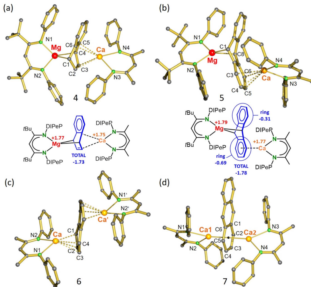
Fig. 1 (a) Crystal structure and NPA charges for (^{\text{DIPePBDI}}\text{BDI}^*)\text{Mg}(\mu^2, \mu^4\text{-naphthalene})\text{Ca}(\text{DIPePBDI}) (4). (b) Crystal structure and NPA charges for (^{\text{DIPePBDI}}\text{BDI}^*)\text{Mg}(\mu^2, \mu^4\text{-anthracene})\text{Ca}(\text{DIPePBDI}) (5). (c) Crystal structure of (^{\text{DIPePBDI}}\text{BDI})\text{Ca}(\mu^4, \mu^4\text{-naphthalene})\text{Ca}(\text{DIPePBDI}) (6). (d) Crystal structure of (^{\text{DIPePBDI}}\text{BDI})\text{Ca}(\mu^6, \mu^6\text{-anthracene})\text{Ca}(\text{DIPePBDI}) (7). All \text{Et}_2\text{CH} -substituents and H atoms have been omitted for clarity. Selected bond distances are summarized in Table 1.
