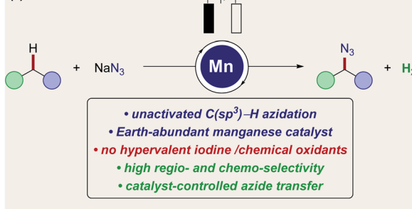
Scheme 1 Manganaelectro-catalyzed azidation.
