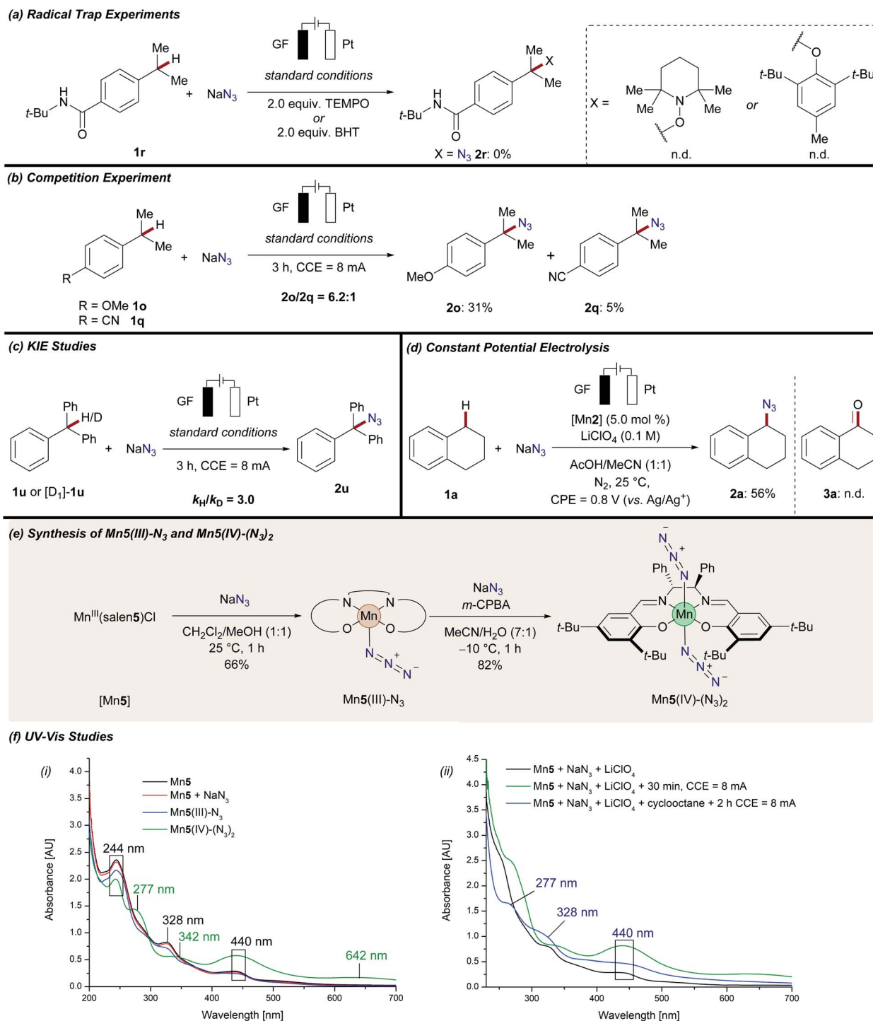
Scheme 5 Mechanistic investigation of manganaelectro-catalyzed azidation of unactivated C(sp 3 )-H bonds. (a) Radical trap experiments. (b) Competition experiment. (c) Kinetic experiments. (d) Chronoamperometric studies at 0.8 V vs. Ag/Ag + . (e) Stoichiometric synthesis of well-defined manganese(III) azide and manganese(IV) diazide complexes. (f) UV-vis spectroscopic studies: (i) MeCN (0.04 mM) was used as the solvent at 25 °C. (ii) MeCN/AcOH (1 : 1, 0.05 mM) was used as the solvent at 25 °C.
