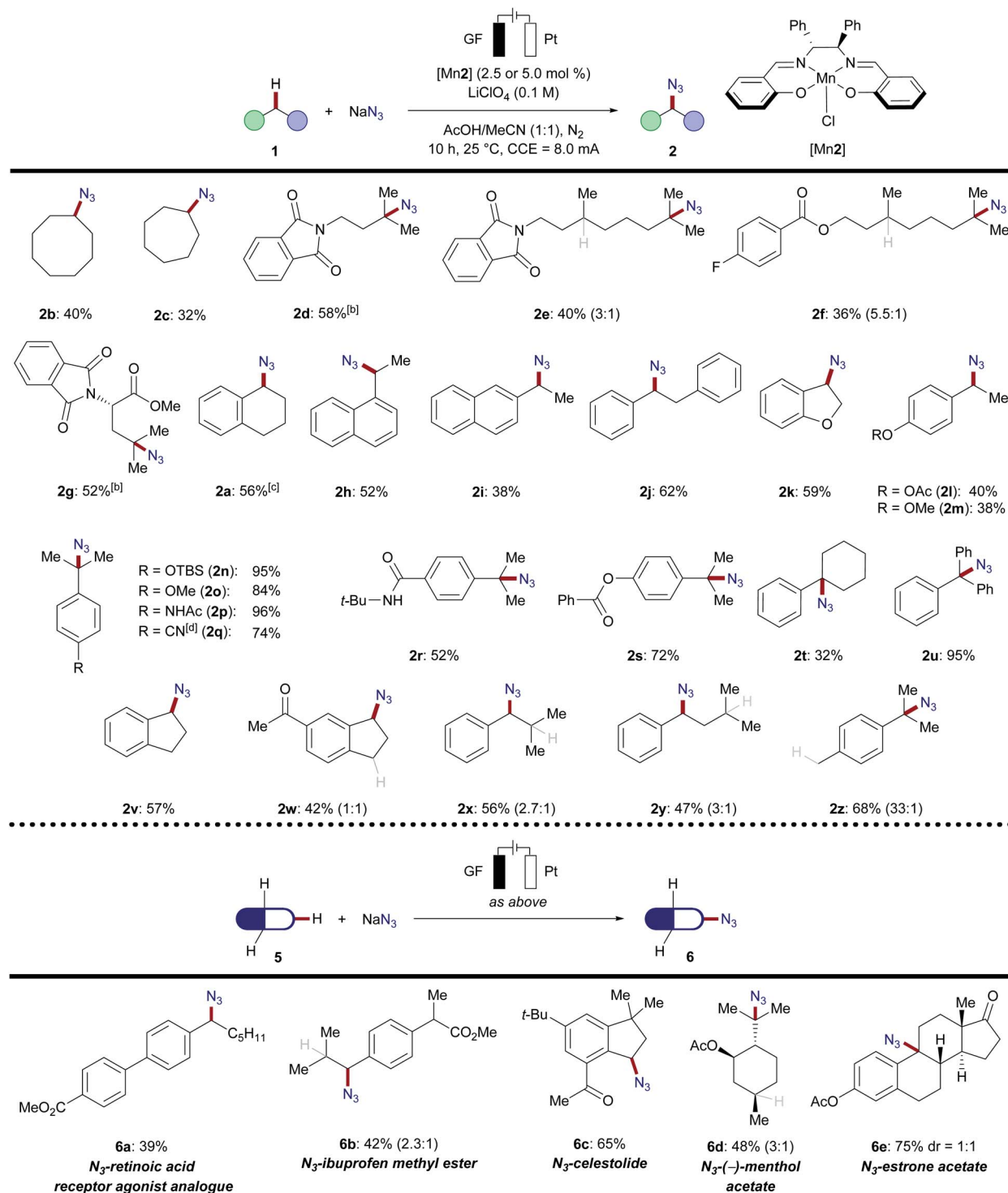
Scheme 3 Reaction scope of manganaelectro-catalyzed \text{C}(\text{sp}^3)\text{-H} azidation. [a] Standard conditions: substrate (0.5 mmol), \text{NaN}_3 (4.0 mmol), [\text{Mn}2] (2.5 or 5.0 mol%), \text{LiClO}_4 (0.5 mmol), \text{MeCN/ACOH} (5 mL, 1 : 1), a nitrogen atmosphere, 10 h, 25 °C, and constant current electrolysis at 8.0 mA in an undivided cell. All yields are isolated products; ratios for site-selectivity are determined by ^1\text{H-NMR} of the crude mixture. [b] At 50 °C. [c] 3,4-Dihydronaphthalen-1(2 H )-one 3 was detected in 10% from crude ^1\text{H-NMR} with 1,3,5-trimethoxy benzene as the internal standard. [d] Standard conditions for 20 h. 32
