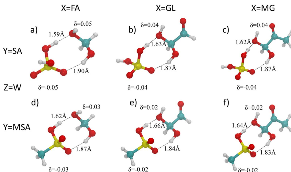
Fig. 3 The most stable structures of X-Y-Z (X = FA/GL/MG; Y = SA/MSA; Z = W) systems at the MP2/6-311+G(d, p)//B3LYP-D3/6-31G(d) level. Yellow, red, green and white spheres represent sulfur, oxygen, carbon and hydrogen atoms, respectively.
