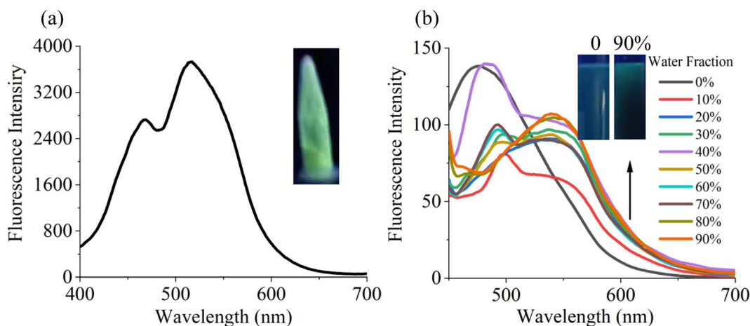
Fig. 1 (a) The emission spectra of probe N in the solid state. (b) Fluorescence spectra of probe N ( 10 \mu\text{M} ) in EtOH/ \text{H}_2\text{O} with different water fractions.
