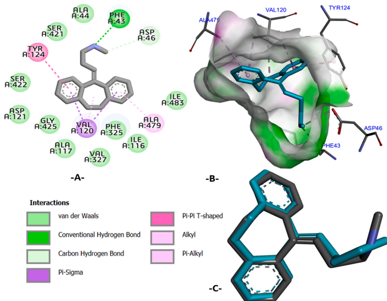
Fig. 8. 2D (A) and 3D (B) visualization of intermolecular interactions created between the docked nortriptyline and 4M48. pdb protein with a binding energy of -8.36 kcal/mol, and re-docking pose (c) defined by a RMSD value of 0.552 Å (docked nortriptyline in cyan and co-crystallized nortriptyline colored by the atomic elements). (The key-colored rectangles show all types of intermolecular interactions, produced between the nortriptyline and the target protein)
