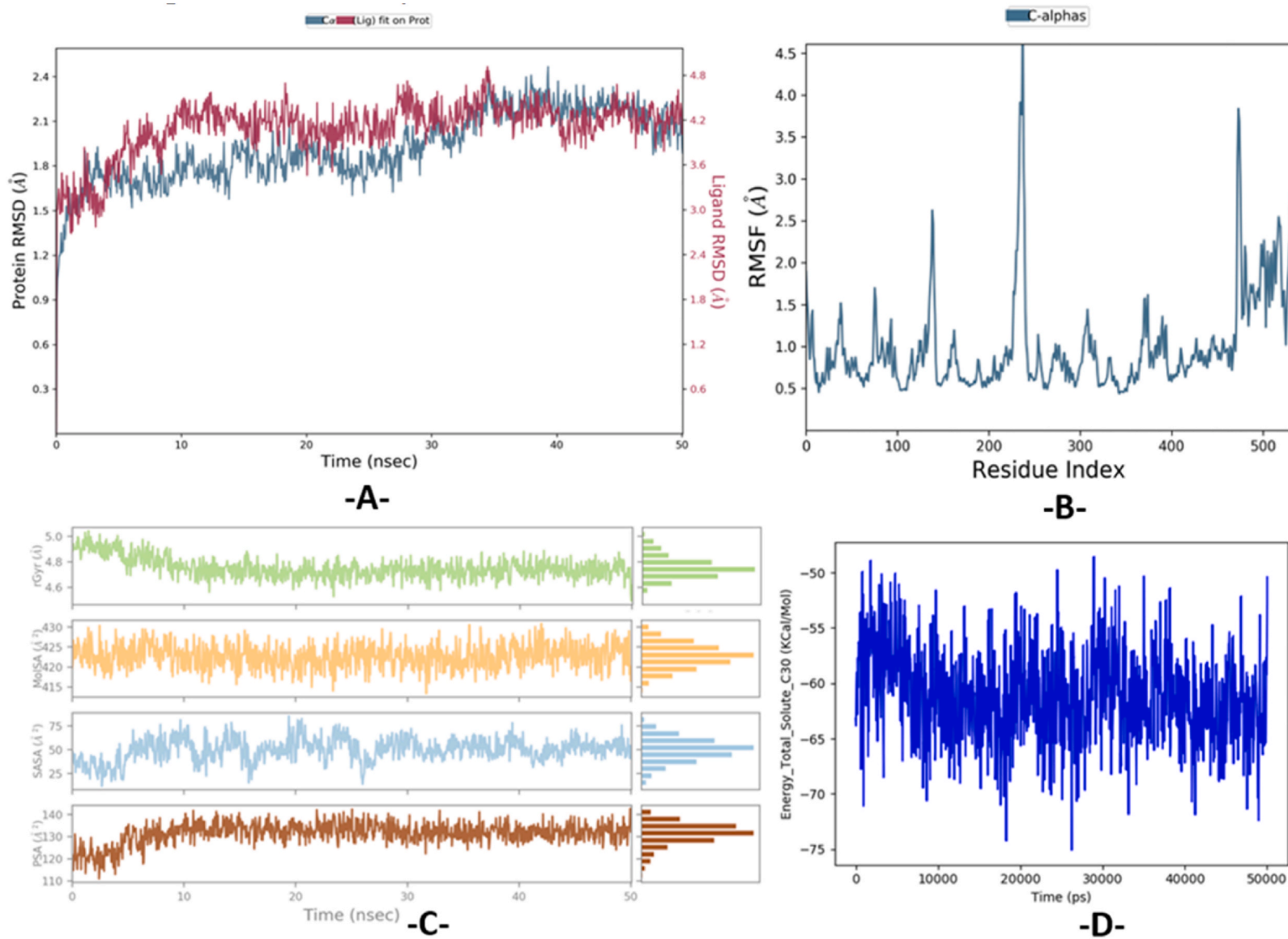
Fig. 10. Evolution of RMSD, RMSF, Rg, MolSA, SASA, PSA, and total free energy during 50 ns, for (L30-DAT protein) complex.
