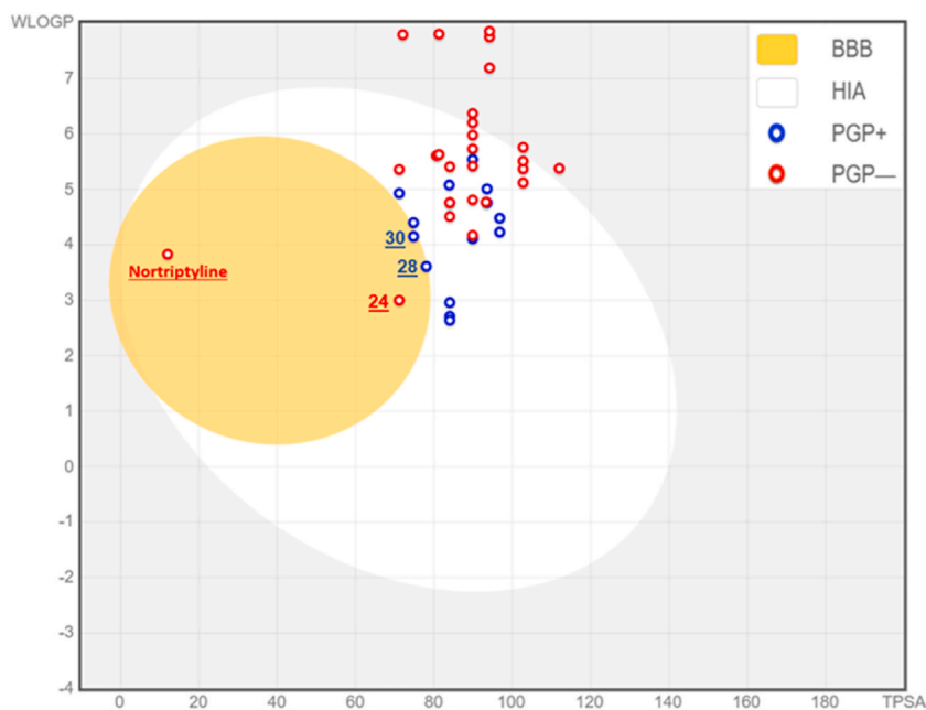
Fig. 5. BOILED-Egg model of nortriptyline and forty pyrrolo [3,4-c]pyrazole and azetidine derivatives. (BBB: blood-brain barrier; HIA: human intestinal absorption; PGP: P -glycoprotein).
