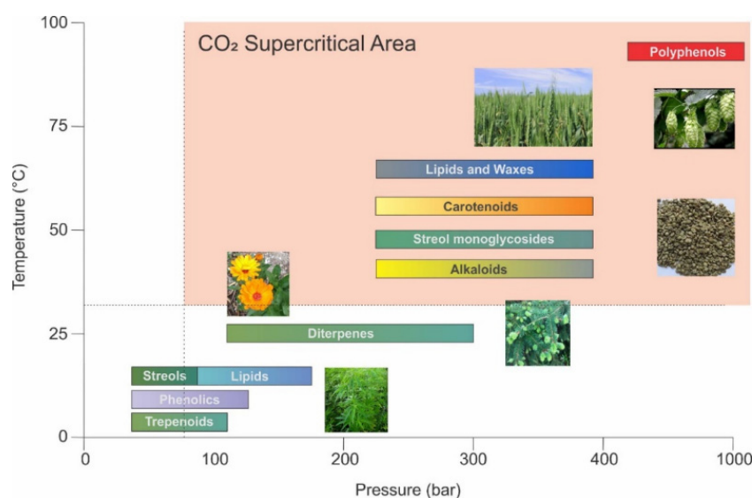
Figure 1. Schematic diagram showing control parameters of Supercritical Extraction (SCE) processes for the extraction of bioactive compounds.
