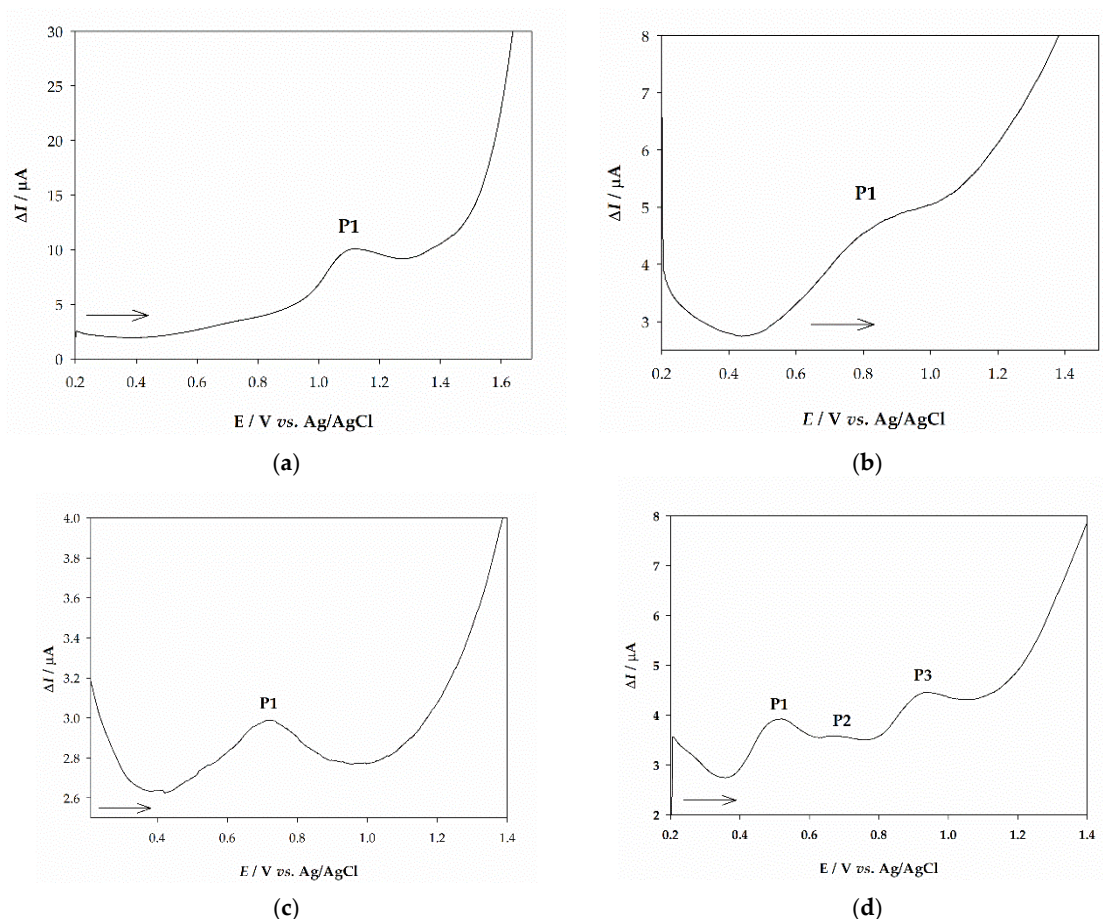
Figure 6. Square-wave voltammograms (SWV) of supercritical CO 2 extracts obtained from four medicinal plants: (a) Chamomile; (b) Yarrow; (c) St. John’s wort; (d) Curry plant in the form of microfilm immobilized on the surface of glassy carbon electrode (GCE) and immersed in Britton Robinson buffer (pH 2.5). The experimental conditions are as depicted in Figure 5.
