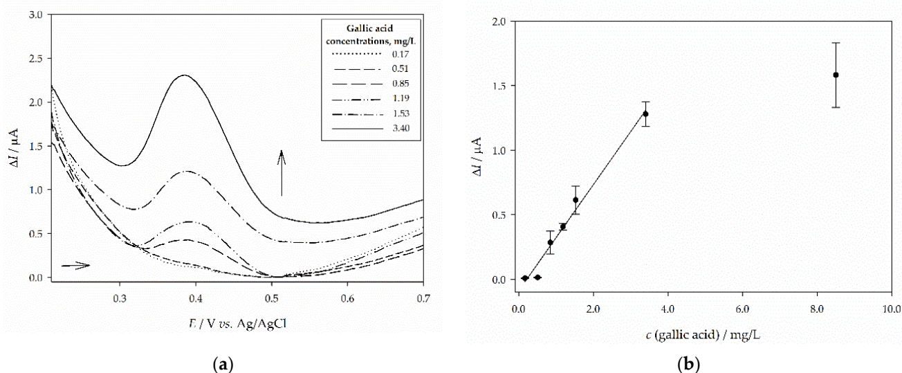
Figure 5. Experimental analysis of polyphenolic standard gallic acid: (a) square-wave voltammograms (SWV) obtained on the surface of glassy carbon electrode (GCE) and immersed in Britton Robinson buffer (pH 2.5) for concentration range 0.17–3.40 mg/L; (b) dependence of the net peak currents on the concentration of gallic acid with the linear regression line. The frequency is 10 Hz, pulse amplitude is 50 mV, and the step potential is 2 mV.
