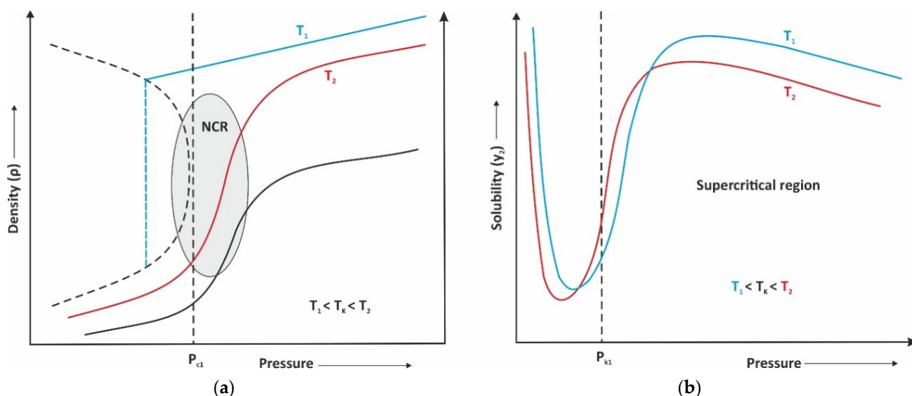
Figure 2. The interconnection between the (a) density and (b) solubility by increasing the pressure.
