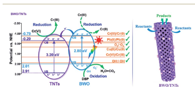
Scheme 2 The synergistic photocatalytic mechanism for \text{Cr}(\text{vi}) -DBP mixed pollutant removal on the BWO/TNTs composite under visible light irradiation.
