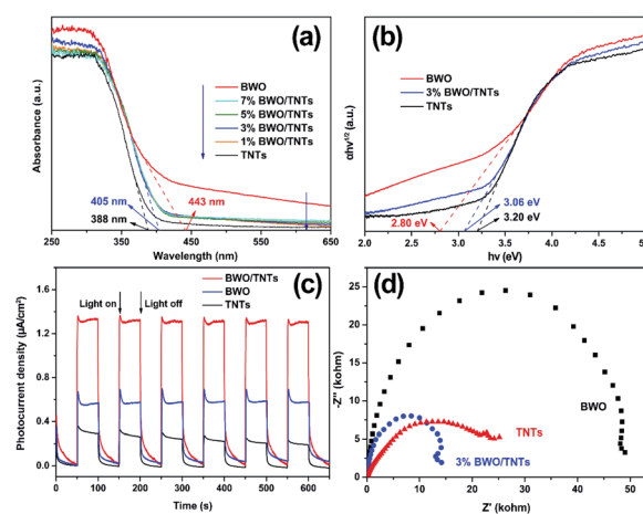
Fig. 5 UV-vis DRS spectra (a), Tauc plots (b), transient photocurrent response curves under visible light irradiation (c), and EIS Nyquist plots (d) of the samples.
