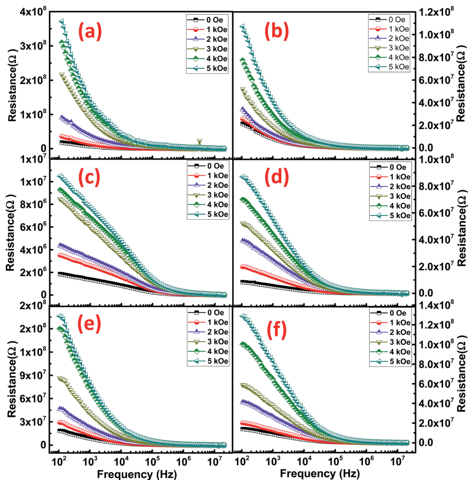
Fig. 9 Variation of resistance with frequency at different magnetic fields for (a) CFO-1, (b) CFO-2, (c) NFO-1, (d) NFO-2, (e) NCF-1 and (f) NCF-2 NRs.
