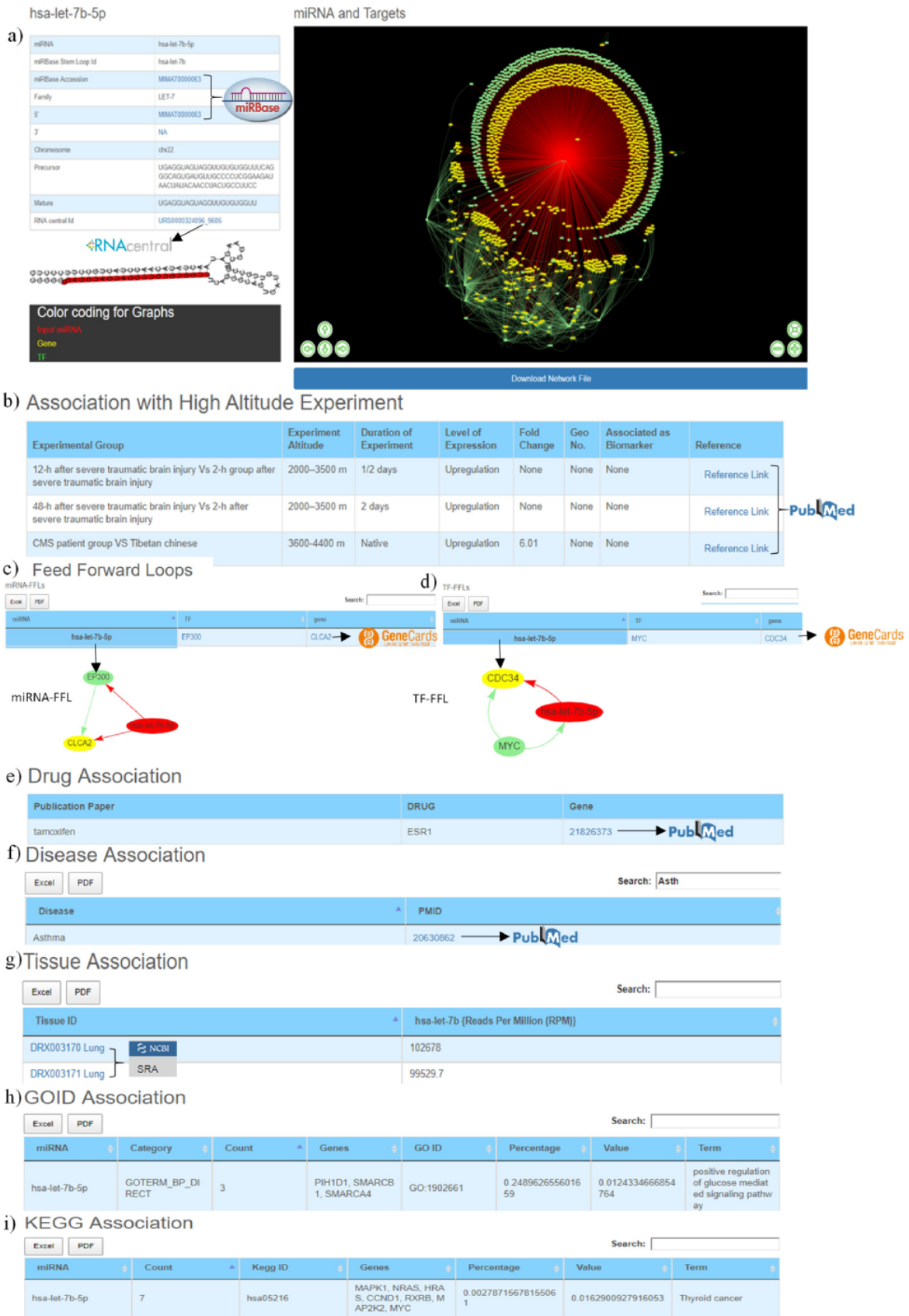
Figure 3. Web image of the miRNA information page. (a) The first section of hsa-let-7b-5p miRNA information page with details about the miRNA and hyperlinking to external databases like miRBase and RNAcentral. (b) The second section shows information related to experimental details of DE human miRNA under HA conditions in published literature. (c) The web image of the miRNA-FFL in tabular format. (d) The web image of the TF-FFL in tabular format. (e) miRNA associations with drug. (f) miRNA associations with different disease. (g) miRNA expression level in different tissues. (h) GO functional enrichment of the miRNA targets. (i) KEGG pathway enrichment of the miRNA targets. The lengthy tables can be searched through 'search' box and information in table can be download in both Excel and PDF formats.
