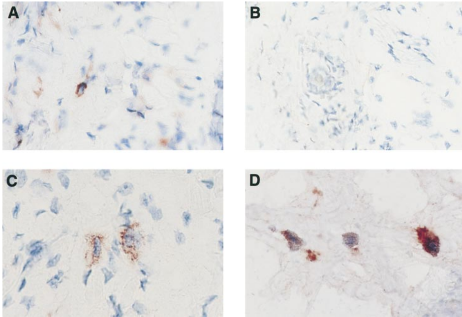
Figure 6. MIP-2 immunoreactivity in tissue mast cells from TNF^{-/-} mice. Kit^W/Kit^{W-v} mice were reconstituted with mast cells from either TNF^{-/-} mice (A and B) or congenic WT mice (C). These animals and, in addition, TNF^{-/-} mice (D), were sensitized and challenged with TNCB. MIP-2 (A, C, and D) immunoreactivity was analyzed in fixed cryosections as described in Materials and Methods. (B) Analysis of immunoreactivity in the absence of the primary Ab. Similarly, no staining was found in the corresponding controls for C and D.
