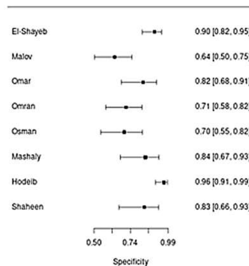
Forest plot of specificity
