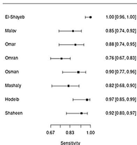
Forest plot of sensitivity
