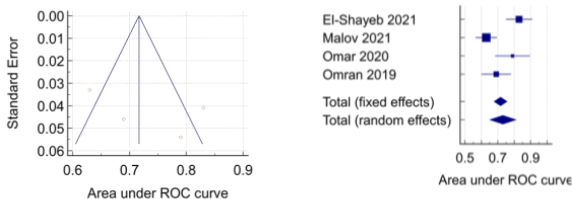
Figure 3. Area under curve analysis of AFP-related studies
