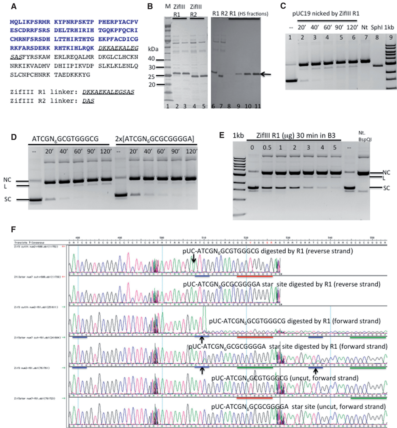
Figure 3. Characterization of Zif268::N.φGamma F5 chimeric nickase (ZifIII). (A) Amino acid sequence of the fusion HNHE (Zif268 sequence shown in blue). The sequence was derived from partial ZFP of Vireo cassinii (GenBank: gb AAO84760). Two fusion constructs were made, R1 with a 13-aa linker (7 aa: DKKAEKA from the native songbird Zif268) and R2 with 3-aa linker between the two functional domains. (B) SDS-PAGE analysis of purified ZifIII R1 and R2 HNHEs. Lanes 2–5, 6 and 7, purified R1 and R2 fusion proteins from chitin columns. Lanes 8–11, purified R1 fusion protein from a heparin column (HiTrap Heparin HP, 5 ml). (C) Nicked pUC19 DNA in a time course (lanes 2 and 6, 20 min to 2 h). Lanes 7 and 8, Nt.BspQI nicked and SphI-digested DNA, respectively. (D) Digestion of pUC-ATCG-N 6 -Zif3(GCGTGGGCG) and pUC-ATCG-N 6 -Zif3star(GCGCGGGGA) in a time course (20 min to 2 h) in Buffer 3 (100 mM NaCl). Small amount of linear DNA (<5% of total DNA) appeared after 20 min digestion. Note: there is a pre-existing ‘star’ site in pUC19 in addition to the cognate site or ‘star’ site inserted at the multiple cloning sites. (E) Digestion of pUC-ATCG-N 6 -Zif3(GCGTGGGCG) by varying concentration of ZifIII R1 in NEB Buffer 3 for 30 min. The Nt.BspQI-nicked DNA was used as a marker. The slow migrating DNA in (E) and (F) is probably nicked dimer. (F) Run-off sequencing of nicked DNA (B3, 1 h, 37°C) with forward and reverse primers. Red line, Zif268 cognate site; green line: Zif268 ‘star’ site; blue line: N.φGamma site. Arrows indicate the nicking sites where double peaks appeared. SC, supercoiled; L, linear; NC, nicked circular DNA.
