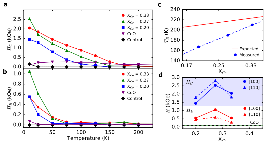
Figure 3. Plot of (a) coercive field and (b) exchange bias field, measured along the [100] crystallographic axis, versus temperature for entropy-stabilized oxide exchange bias heterostructures containing varying compositions of Co, plotted with a Pt/Py/CoO/MgO heterostructure (labeled CoO in the figure) and Pt/Py/MgO control sample. (c) The blocking temperatures ( T_B ) extracted from Sup. Figure 9 (Measured), along with our prediction using the rule of mixtures (Expected), obtained by taking a weighted average of the individual Néel temperatures of the constituent binary oxides. The blocking temperature deviates significantly from the rule of mixtures, but approaches the expected value as the concentration is increased. The dashed line is provided as a guide to the eye. (d) Plot showing the change in coercive ( H_C ) and bias ( H_B ) fields as a function of Co concentration along both the [100] and [110] crystallographic directions at 10 K. The dashed line at 0.075 kOe corresponds to the bias field in the Pt/Py/CoO/MgO control sample. Error bars are smaller than the points for all plots.
