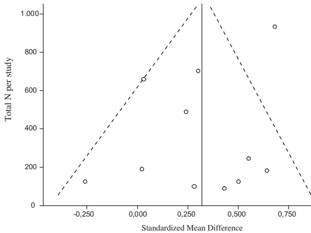
Fig. 3. Funnel plot with total N/study on the y-axis, effect size for PTSD on the x-axis and an indicator line for the pooled Standardized Mean Difference.
