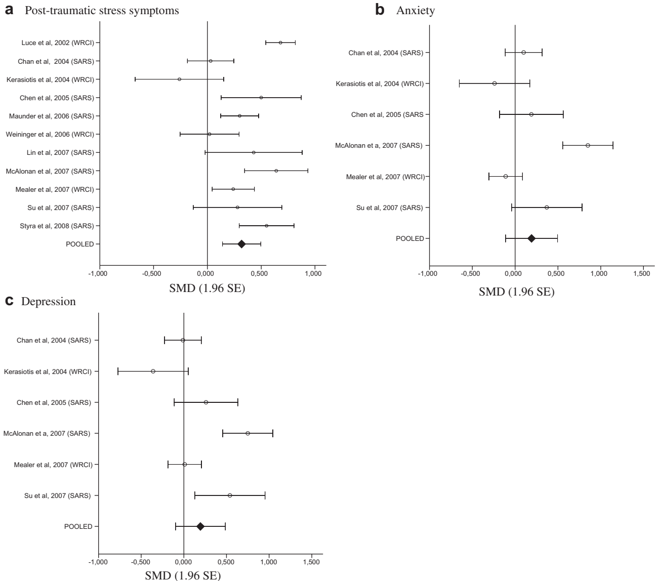
Fig. 2. a–c Effect size, in terms of standardized mean differences (SMDs) with 95% Confidence Intervals, of work-related critical incidents on post-traumatic stress symptoms ( k = 11 ), anxiety ( k = 6 ), and depression ( k = 6 ), as well as the pooled effect on the three outcomes.
