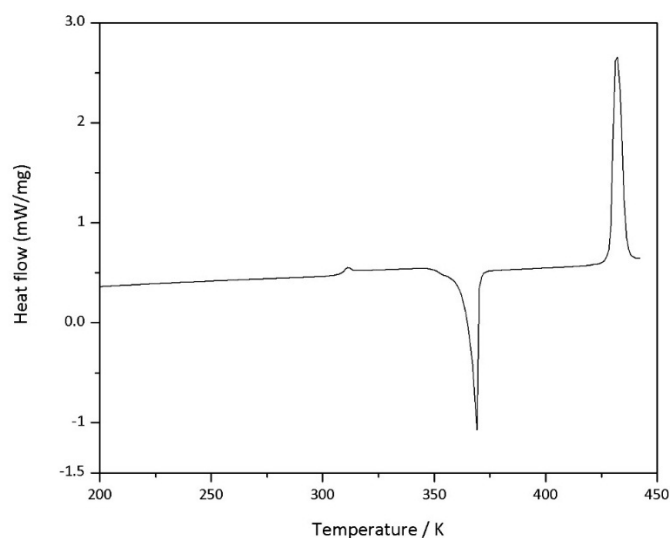
Figure 8. Second DSC scan from (\text{EtPh}_3\text{P})_2[\text{CuBr}_4] (7).
