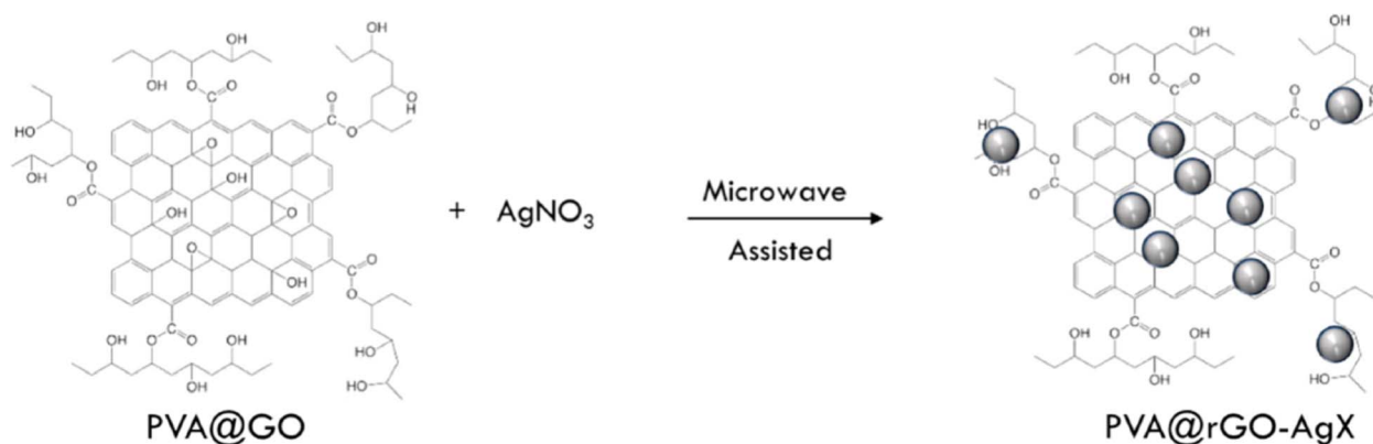
Fig. 2 A diagram illustrating the process of creating hybrid systems made of PVA GO and silver denoted as PVA@rGO-AgX. Reproduced with permission. 57 Copyright 2020 by the authors. Licensee MDPI, Basel, Switzerland.
