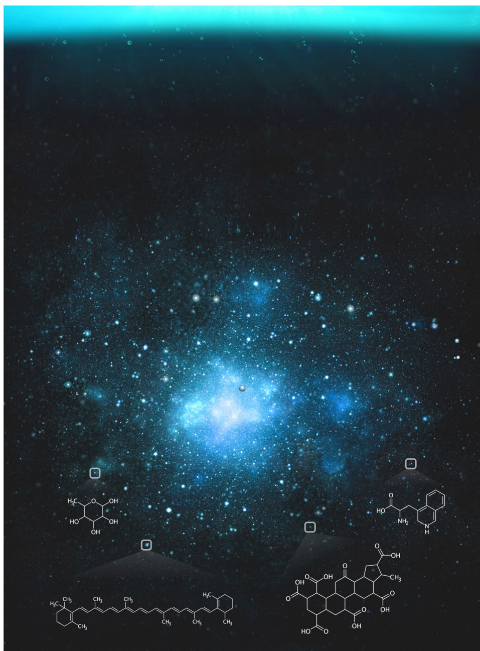
Fig. 1 A molecular universe in the ocean. This illustration depicts the molecular complexity of marine DOM. Most of this pool is chemically unidentified (big nebulous), with only 2–3% of defined chemical structures (gray squares). The representative structures of marine DOM namely carotenoids, carboxylic-rich alicyclic molecules, and fucose were extracted from Arakawa et al. (2017), Hertkorn et al. (2006), and Repeta (2015), respectively
