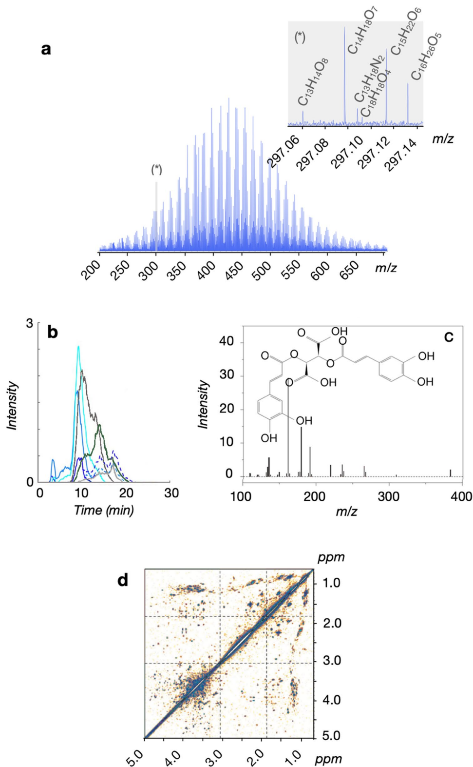
Fig. 2 More than ten thousand molecular formulas and structural units have been identified in marine DOM. a A mass spectrum measured via ultrahigh-resolution mass spectrometry (15 T Fourier transform ion cyclotron resonance mass spectrometry, FT-ICR-MS) of the North Pacific Equatorial Intermediate Water with single asterisk indicating exemplary nominal mass (297 Da). b An HPLC–MS/MS scan of isomeric mixture peaks from Nordic Reservoir natural organic matter (NRNOM) reference material, depicting the inability to distinguish fragmentation patterns from individual isomers from a molecular mass (adapted from Hawkes et al. 2018). c An example of an assigned structure (C 22 H 18 O 12 ) based on a riverine DOM MS/MS spectra and the METLIN database (adapted from Lu and Liu 2019). d The structural units identified by multidimensional nuclear magnetic resonance (NMR), in which each dot represents one structural feature (Hertkorn et al. 2012)
