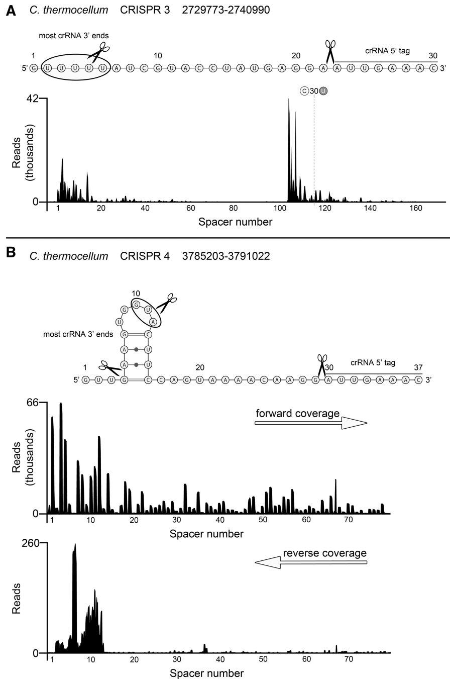
Figure 2. crRNA processing in C. thermocellum . Illumina HiSeq2000 sequencing reads were mapped to the C. thermocellum ATCC 27405 reference genome and selected CRISPR regions are displayed. Conserved 5'-terminal crRNA cleavage sites and variably trimmed 3'-termini are indicated within the repeat sequence. A possible hairpin structure was predicted by RNAfold (41). All C. thermocellum CRISPR mappings are found in Supplementary Figure S2. (A) CRISPR locus 3 reveals internal promotion of crRNA transcription at Spacer 104. (B) CRISPR locus 4 exemplifies bidirectional CRISPR transcription. Forward and reverse reads were separated to highlight the occurrence of processed anti-crRNAs that can correlate with reduced crRNA abundance.
