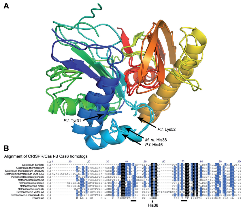
Figure 3. Structural model of Cas6b shows high similarity to Pf Cas6. (A) A structure model (I-Tasser) of M. marisplacidus Cas6b was aligned to Pf Cas6 (DaliLite). The catalytic site of Pf Cas6 is indicated and a histidine at Position 38 in Cas6b is located in close proximity to the catalytic histidine in P. furiosus . (B) An alignment of Cas6b homologues (ClustalW) of subtype I-B shows conserved amino acid residues (black coloured residues) and reveals putative catalytic residues (black bars).
