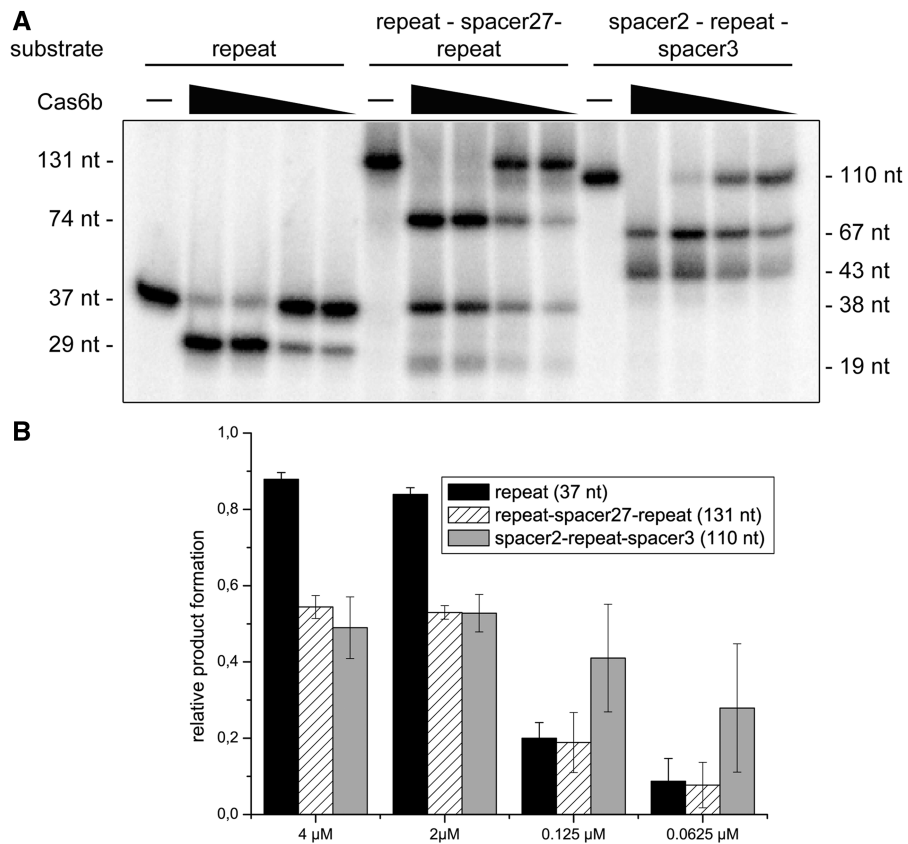
Figure 5. RNA substrates for Cas6b processing. The two ‘repeat-spacer27-repeat’ and ‘spacer2-repeat-spacer3’ substrates were internally labelled by in vitro transcription and repeat RNA molecules were 5'-end labelled. The substrates were used in three independent cleavage assays using different concentrations of Cas6b (4, 2, 0.125 and 0.0625 μM). (A) A representative assay shows the ability of Cas6b to process all used substrates in similar manner and efficiency. (B) Product formation for three independent reactions was quantified.
