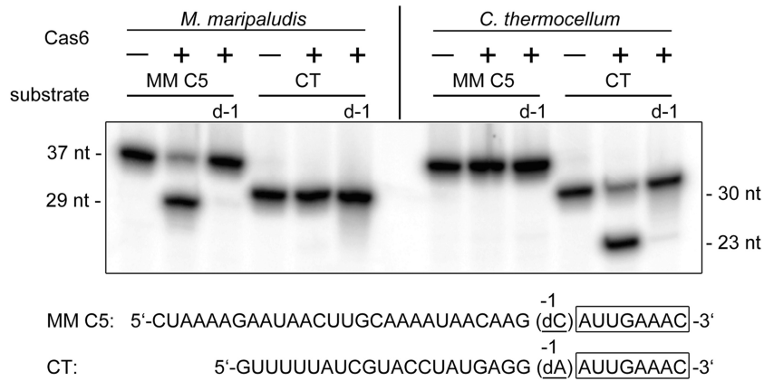
Figure 4. Cas6b of M. maripaludis (MM C5) and C. thermocellum Cthe_2303 (CT) cleave their specific repeat structure. Cas6b endonuclease assays were performed with 5'-terminal radioactively labelled repeat RNA and the respective deoxy variants (indicated at the bottom, -1 displaying the first base upstream of the 5'-tag) of M. maripaludis and C. thermocellum . Cas6b processes the 37-nt repeat into the smaller 29-nt fragment, while the deoxy variant (d-1) and the 30-nt repeat RNA of C. thermocellum are not cleaved. Cthe_2303 is specific for its 30-nt repeat RNA.
