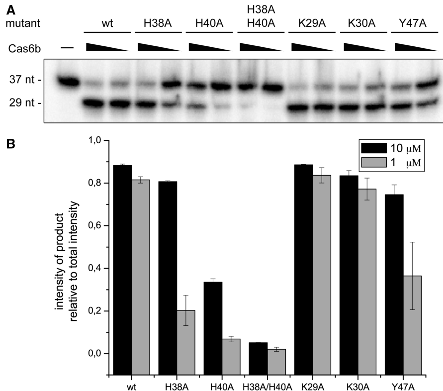
Figure 6. Two histidine residues play a critical role for Cas6b activity. Cas6b endonuclease assays were performed with the indicated Cas6b variants and 5'-end-labelled repeat RNA substrates. (A) A representative assay shows the activities of the Cas6b variants. While mutation of two lysines at Position 29 and 30 did not show any influence on activity in comparison to wild-type (wt), a mutation of two histidines at Positions 38 and 40 as well as a mutation of tyrosine at Position 47 show reduced processing activity. (B) Product formation for three independent reactions was quantified.
