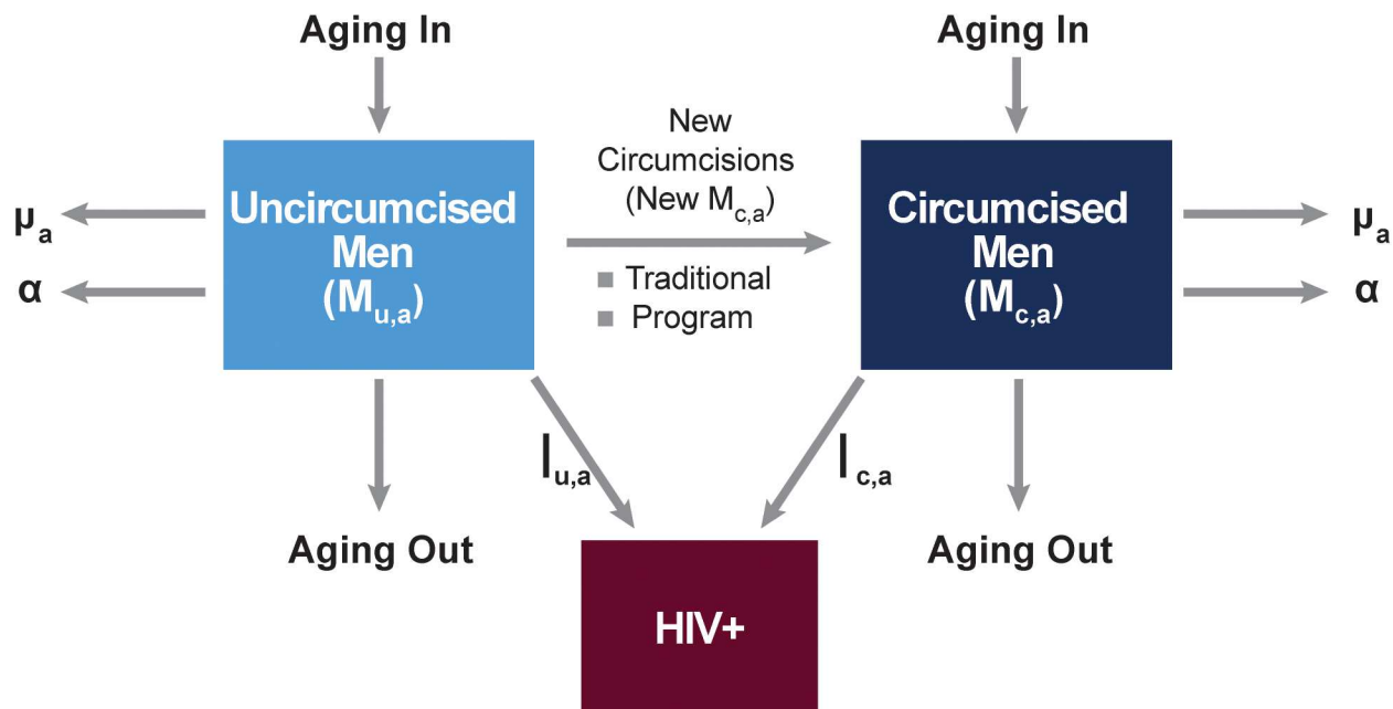
Fig 1. Structure of the DMPPT 2.0 model. \mu_a , non-AIDS mortality; \alpha , AIDS-related mortality; I_{u,a} , HIV incidence of uncircumcised men; I_{c,a} , HIV incidence of circumcised men.
