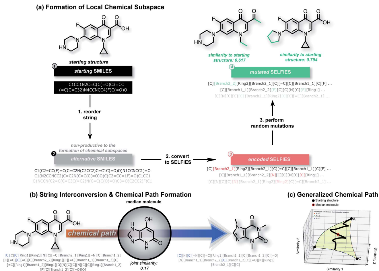
Fig. 1 Illustration of string manipulations within STONED to form local chemical subspaces (a, see Section II B) for a given structure, discovering median molecules on the chemical path between two structures (b, see Section II C) and formation of generalized chemical paths between more than two molecules (c, see Section II D).
