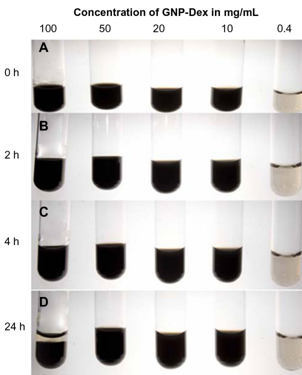
Figure 3 Digital images of vials containing graphene nanoplatelets intercalated with manganese ( Mn^{2+} ) ions, functionalized with dextran (GNP-Dex) in water (with mannitol) at 100.0, 50.0, 20.0, 10.0, 0.4 mg/mL concentrations at (A) 0 hour (h), (B) 2 hours, (C) 4 hours, and (D) 24 hours after preparing the solutions.
