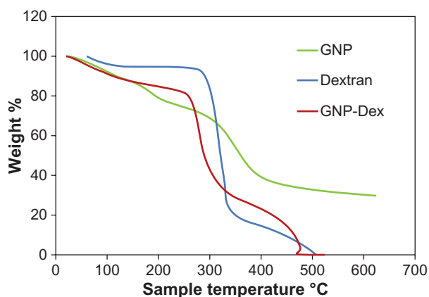
Figure 2 Representative thermogravimetric analysis (TGA) curve of graphene nanoplatelets, dextran, and graphene nanoplatelets intercalated with manganese ( Mn^{2+} ) ions, functionalized with dextran (GNP-Dex).
