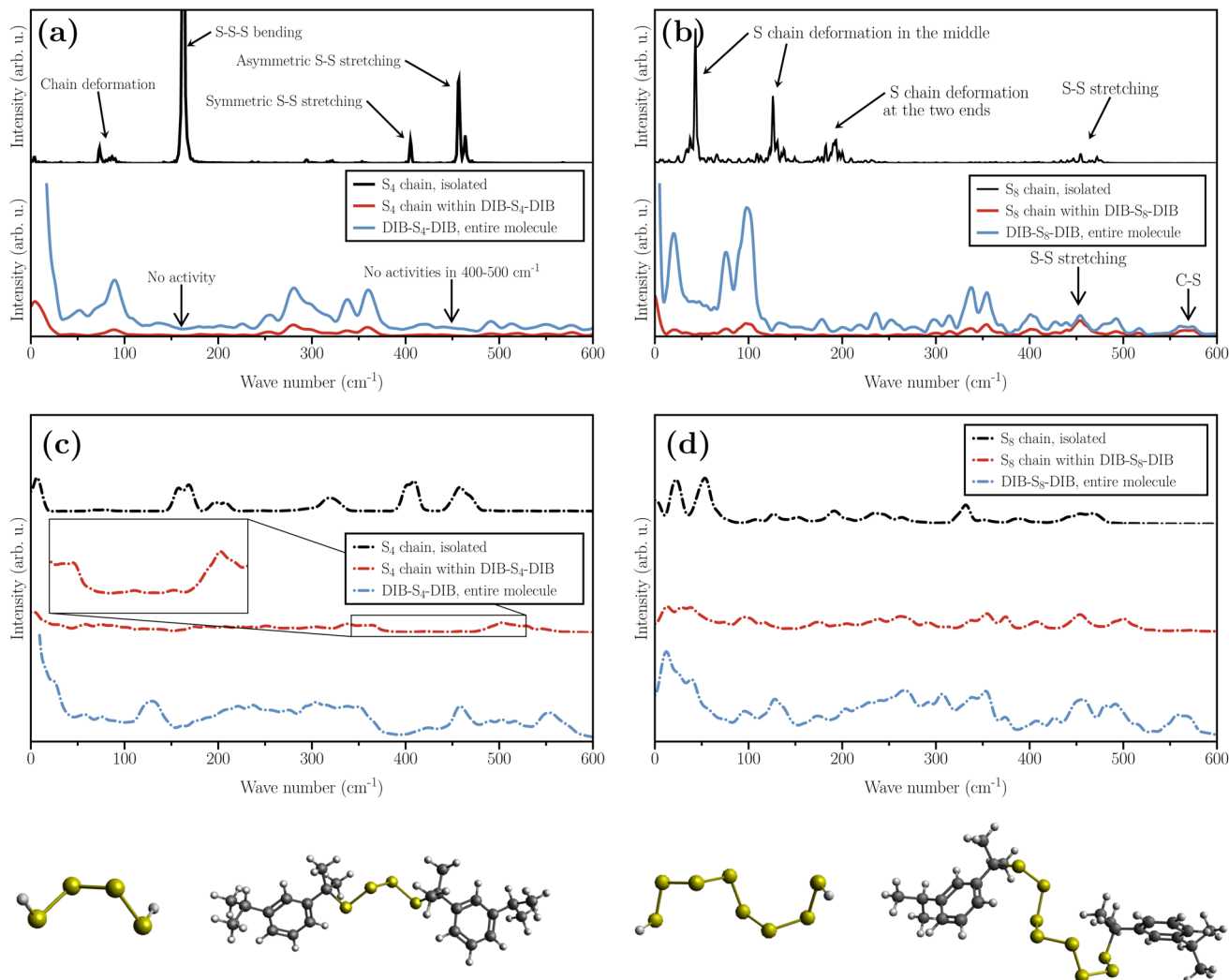
Fig. 2 Calculated Raman spectra of (a) DIB- S_4 -DIB and (b) DIB- S_8 -DIB in vacuum. Also shown in (a) and (b) are the computed Raman spectra of isolated S_4 and S_8 chains (black curves). Partial Raman spectra arising from sulfur chains within DIB- S_4 -DIB and DIB- S_8 -DIB systems are shown in red curves. (c) and (d) show the computed power spectra of DIB- S_4 -DIB and DIB- S_8 -DIB, respectively (blue curves). Power spectra of isolated S_4 and S_8 chains are shown in black, while partial power spectra of sulfur chains are shown in red curves. Minimum-energy structures of isolated S_4 and S_8 chains as well as those of DIB- S_4 -DIB and DIB- S_8 -DIB molecules are shown also in the lower panel.
