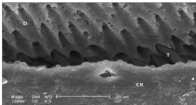
Figure 3: Standard error mean image of interface of (OptiBond Solo Plus + LS Bond) and dentin ( \times 1250 ). CR: Composite resin; T: Resin tag; D: Dentin.
