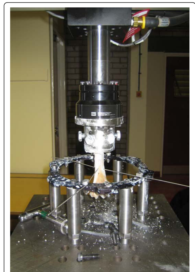
Figure 2 A typical test setup using transverse wires.
