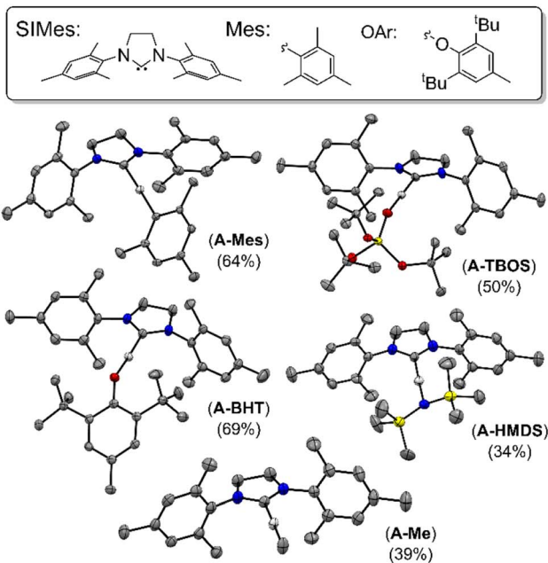
Scheme 2 Synthesis of molecular compounds of general structure (SIMes)AgX via salt metathesis (a) and protonolysis (b). (Ar = 2,6-( t Bu)-4-(Me)-C 6 H 2 ). Crystal structures of all crystallized complexes and corresponding yields. (TBOS = -OSi(O t Bu) 3 , HMDS = -N(SiMe 3 ) 2 ) (crystal structures depicted at 50% probability with the exception of A-HMDS which has ellipsoids at 25% probability for better visibility).
