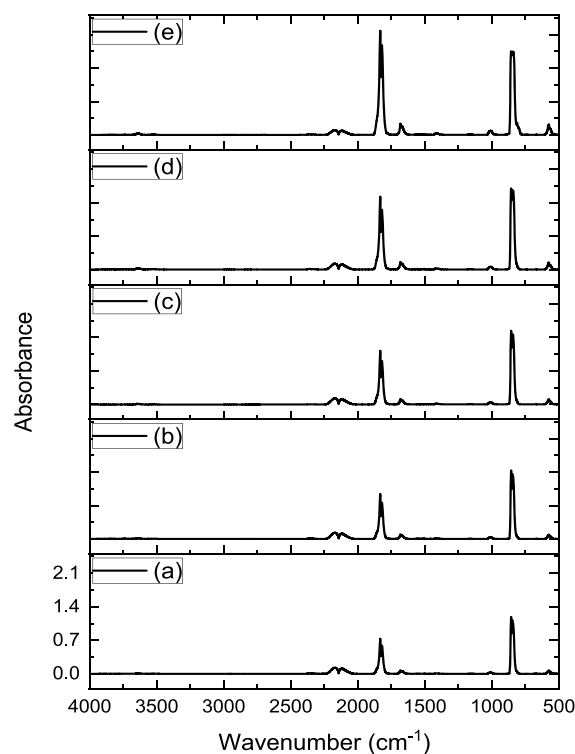
Figure 3. Infrared spectra for the reaction of CO and \text{Cl}_2 over activated carbon at 323 K ( \text{CO} 1.78 \text{ mmol min}^{-1} \text{ g}_{\text{cat}}^{-1} , \text{Cl}_2 1.38 \text{ mmol min}^{-1} \text{ g}_{\text{cat}}^{-1} in a total flow of 159 \text{ cm}^3 \text{ min}^{-1} ) as a function of \text{Br}_2 flow rate: (a) 0, (b) 2.99 \times 10^{-3} , (c) 5.6 \times 10^{-3} , (d) 1.31 \times 10^{-2} , and (e) 1.99 \times 10^{-2} \text{ mmol Br}_2 \text{ min}^{-1} \text{ g}_{\text{cat}}^{-1} . Spectrum (a) is a baseline measurement that is performed with the isolated \text{Br}_2 doser.
