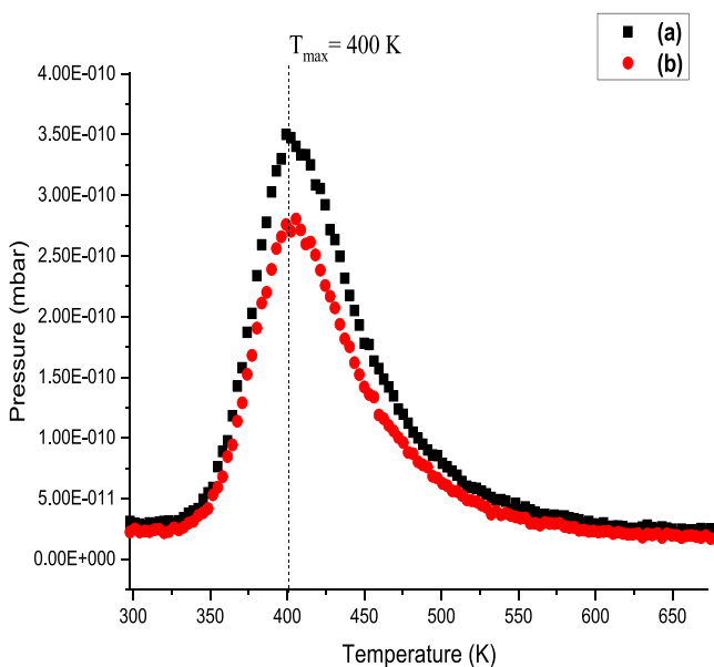
Figure 7. Temperature-programmed desorption profile for activated carbon after Br 2 exposure at 298 K under an incident flow rate of 0.013 mmol Br 2 min -1 g cat -1 up to the point when a Br 2 breakthrough was observed. The incident gas flow into the gas cells was 159 cm 3 min -1 (carrier gas 50 cm 3 N 2 min -1 , diluent post reactor 100 cm 3 N 2 min -1 ). (a) 79 and (b) 81 amu.
