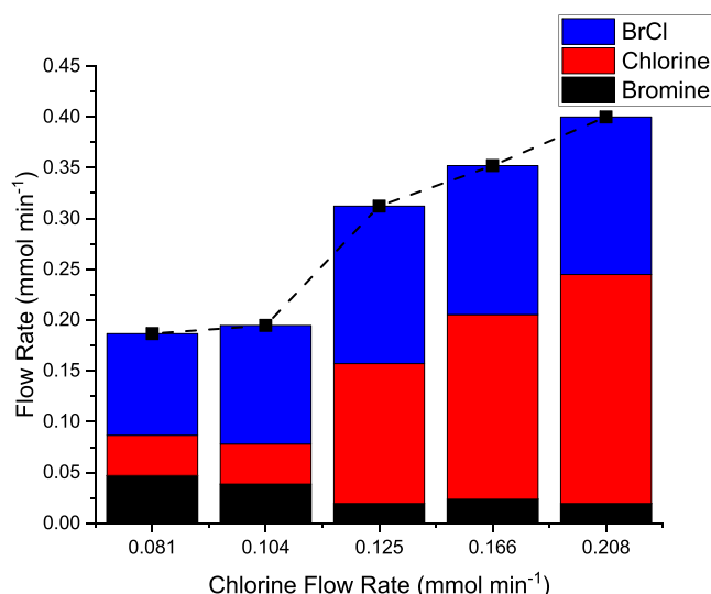
Figure 2. A mass balance plot for varying combinations of \text{Cl}_2 and \text{Br}_2 passed over 0.12 g of ground quartz ( 250\text{--}500 \mu\text{m} size fraction) at 293 K and ambient pressure. The \text{Br}_2 flow rate was kept constant at 0.122 \text{ mmol min}^{-1} , while the \text{Cl}_2 flow rate was increased from 0.081 to 0.208 \text{ mmol min}^{-1} . Incident carrier gas = 54\text{--}57 \text{ cm}^3 \text{ N}_2 \text{ min}^{-1} , diluent post-reactor = 100 \text{ cm}^3 \text{ N}_2 \text{ min}^{-1} , and total flow rate into gas cells = 159 \text{ cm}^3 \text{ min}^{-1} . The \text{Cl}_2 , \text{Br}_2 , and BrCl flow rates were determined from the UV–visible absorption spectra. The black squares present the total incident molar flow rates of \text{Cl}_2 plus \text{Br}_2 .
