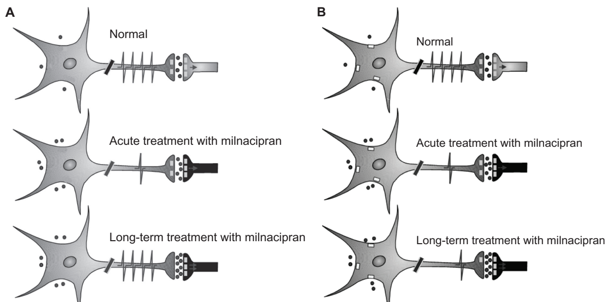
Figure 2 Scheme of the activity of 5-HT (A) and norepinephrine (NE) (B) neurotransmission during treatment with milnacipran. A ) 5-HT system. Acute treatment with milnacipran results in a decreased firing of 5-HT neurons from the raphe nucleus possibly due in part to increased stimulation of somatodendritic autoreceptors. Long-term treatment with milnacipran results in a full recovery in the firing rate of 5-HT neurons in the presence of milnacipran thereby leading to a net increase in 5-HT neurotransmission. Contributing to this enhancement are: 1) the normalized firing rate of 5-HT neurons in the presence of milnacipran 2) the desensitization of the terminal 5-HT 1B autoreceptor, and 3) the desensitization of the \alpha_2 -adrenergic heteroreceptors on 5-HT terminals. B ) NE system. Acute treatment with milnacipran results in increased synaptic concentrations of NE but decreased firing of the NE neurons of the locus coeruleus due to increased stimulation of the somatodendritic \alpha_2 -adrenergic autoreceptors. Long-term treatment with milnacipran results in a further increase in synaptic concentrations of NE due to desensitization of presynaptic autoreceptors. The somatodendritic \alpha_2 -adrenergic autoreceptors do not desensitize.
