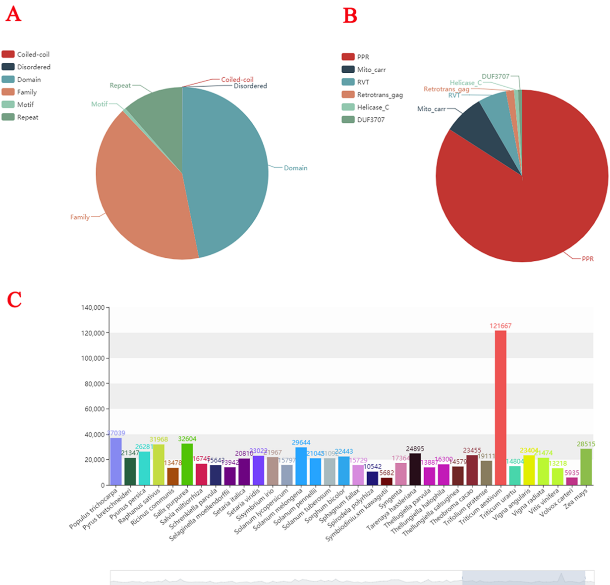
Figure 2. Statistics of plant gene families. (A) The composition structure of 138 plant species' genes. (B) Statistics of the largest number of gene families in each species. (C) The number of gene families of each species.
