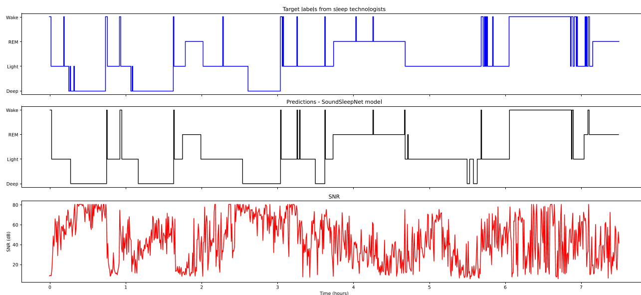
Figure 7 A comparison of the one-night prediction of SoundSleepNet and the PSG result on a subject from the PSG audio test set. The top figure shows target labels given by sleep technologists. The bottom figure shows SNR (dB) of audio signals. The middle figures show predictions of the model.
