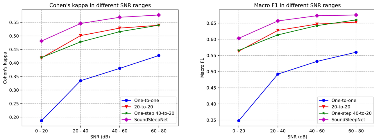
Figure 9 Performances of SoundSleepNet and its counterparts in different SNR ranges.
