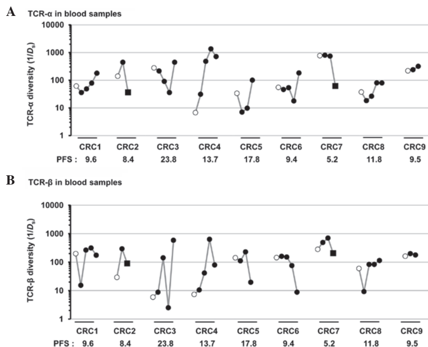
Figure 3. Diversity of the TCR clonotype in blood from 9 patients with CRC. (A) TCR- \alpha and (B) TCR- \beta diversity in blood samples at multiple time points in 9 patients with CRC. Open circles, closed circles and closed squares indicate the time points of pre-treatment, post-treatment and following surgery, respectively. TRC, T cell receptor; CRC, colorectal cancer; PFS, progression-free survival; 1/D_n , inverse Simpson's diversity index.
