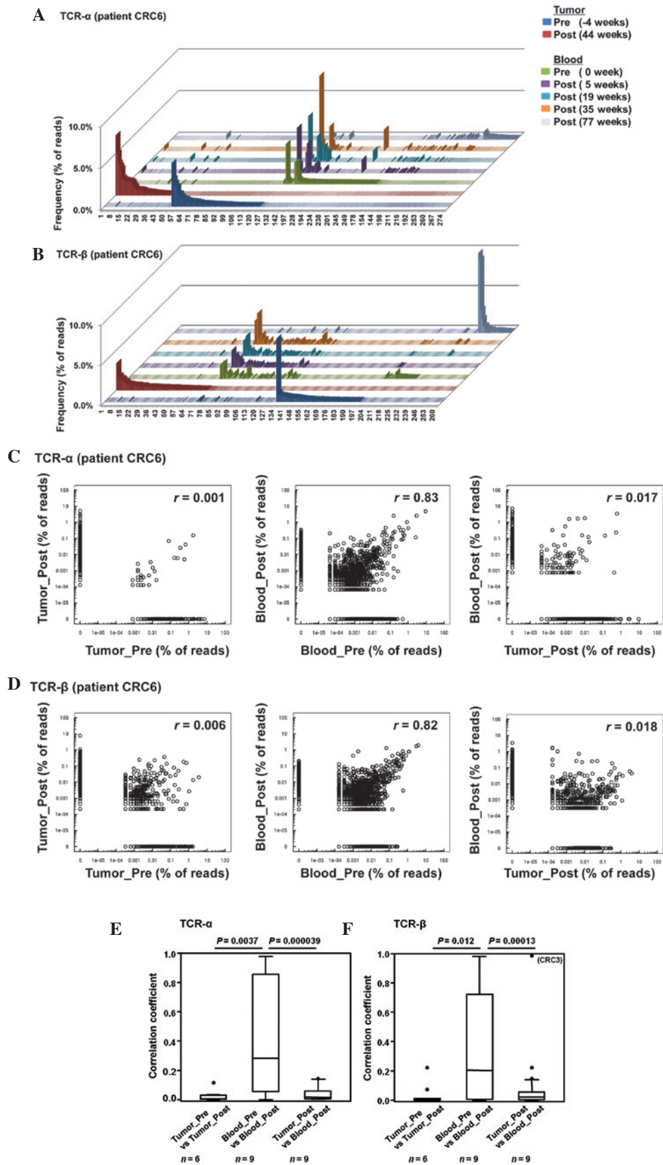
Figure 1. Distribution of the TCR clonotype in tumor tissues and blood of 9 patients with CRC. Frequency distribution of clonotypes of (A) TCR-α and (B) TCR-β in tumor tissues and blood samples from patient CRC6. Clonotypes with functional CDR3 identified at >0.1% in at least one sample were plotted. The frequency was calculated based on the total reads, which include non-functional CDR3. Clonotype frequency plots of (C) TCR-α and (D) TCR-β in patient CRC6. Each dot on the scatter plots indicates a single clonotype with a normalized log 10 clone count graphed at pre-treatment tumor tissue vs. post-treatment tumor tissue (left), pre-treatment blood vs. post-treatment blood (middle) and post-treatment tumor tissue vs. post-treatment blood (right). Blood sample at 35 weeks was used as post-treatment blood. Comparison of the correlation coefficient calculated in (E) TRC-α and (F) TRC-β clonotype frequency plots of 9 patients with CRC. The horizontal line indicates the median concentration, the box covers the 25-75 percentiles and the maximum length of each whisker is 1.5 times the interquartile range. Each dot indicates an outlier. TRC, T cell receptor; CRC, colorectal cancer; CDR3, complementarity determining region 3.
