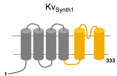
Kv_{Synth} consists of the C-VSP VSD coupled to Kcv. (From Arrigoni et al., 2013.)
