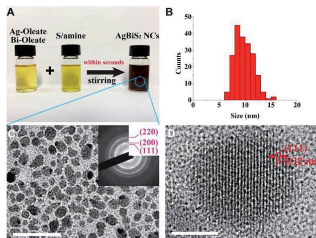
Fig. 1 Characterizations of the \text{AgBiS}_2 NCs synthesized by OA/DDA. (A) Photograph of the Ag/Bi-oleate, sulfur in amine and the \text{AgBiS}_2 NCs. (B) Size distribution profile of the \text{AgBiS}_2 NCs. (C) TEM image of the \text{AgBiS}_2 NCs. Scale bar is 50 nm. Inset: SAED pattern. (D) High resolution TEM image of a single \text{AgBiS}_2 NC. Scale bar is 5 nm.
