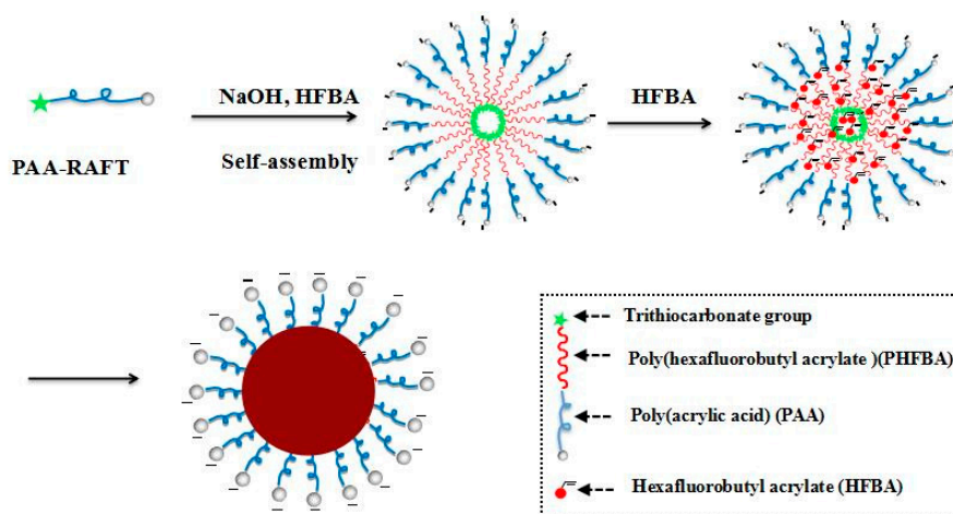
Scheme 2. Reaction scheme for the synthesis of poly(acrylic acid)- b -poly(hexafluorobutyl acrylate) with PAA macro-RAFT agent as stabilizer.
