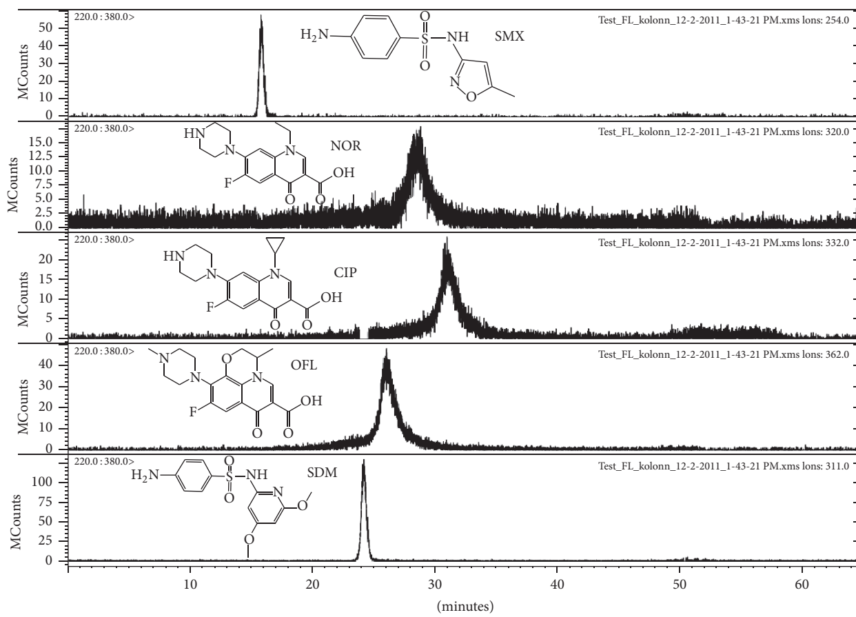
FIGURE 2: MS chromatogram for the standard solution of FQs and SAs ( 10 \mu\text{g/g} ). Eluent: (ammonium acetate, formic acid pH 2.8) and MeOH. Used analytical column: Epic FO-LB C8 column ( 150 \text{ mm} \times 3 \text{ mm} , 3.5 \mu\text{m} ).
