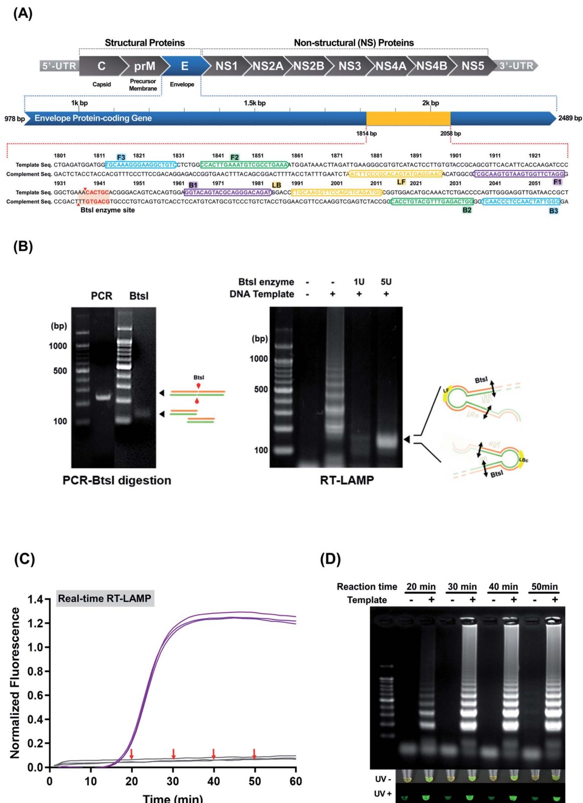
Fig. 1 (A) Specific LAMP region for amplifying the ZIKV envelope protein-coding gene (colored in yellow). (B) Bst I-digested RT-LAMP amplicons. The PCR dsDNA ZIKV products (left panel) and Bst I-digested RT-LAMP amplicons (right panel) were run on an agarose gel; the black arrows indicate Bst I-digested DNA products (120 bp). (C) and (D) Real-time RT-LAMP and agarose gel analysis. Of the four reaction durations (20, 30, 40, and 50 min) attempted, the 40 min reaction was deemed sufficient for ZIKV detection. No false-positive amplifications were observed in the non-template control.
