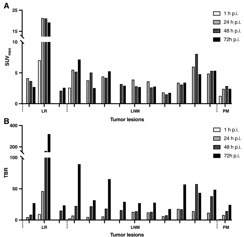
Fig. 4 SUV max (A) and tumor-to-background ratio (TBR) (B) of all tumor lesions at 1 h, 24 h, 48 h, and 72 h post injection (p.i.) of [ 89 Zr]Zr-PSMA-617. LR, local recurrence; LNM, lymph node metastasis; PM, peritoneal metastasis
